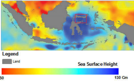
Figure 3-3: Grid data from August 22 nd 2013 after IDW interpolation
