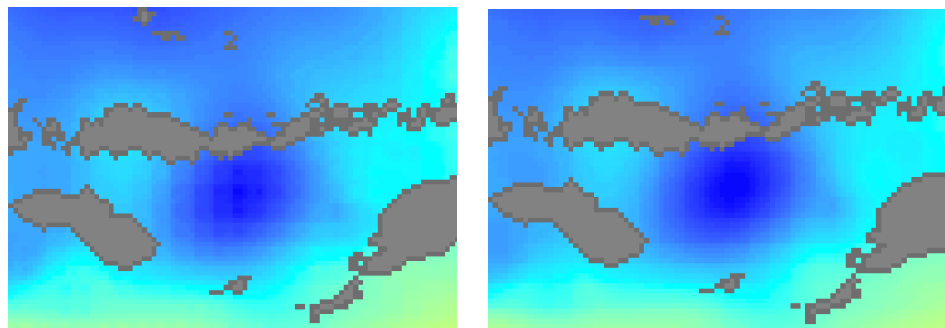
Figure 3-8: Interpolation roughness from IDW (left) and Ordinary Krigging (right)
