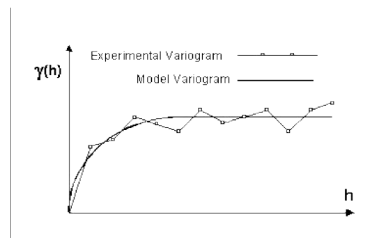
Figure 2-1: Experimental and Model Variogram Used in Kriging
