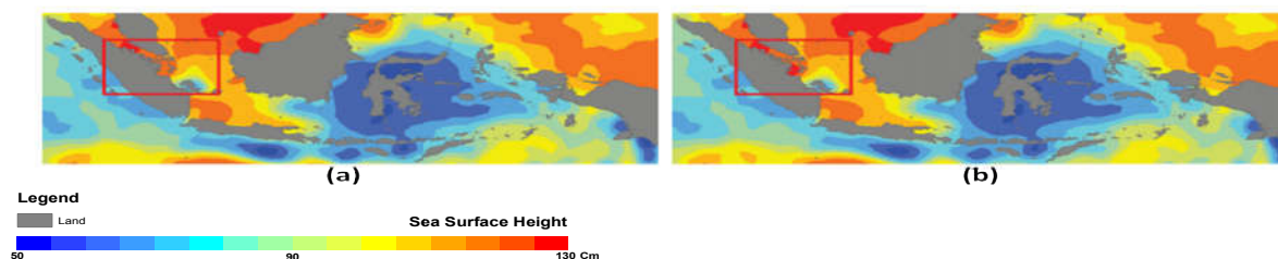
Figure 3-7: Interpolation results from August 25 th 2013, a. IDW; b. Ordinary Krigging
