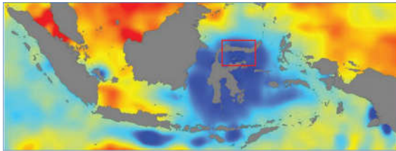
Figure 3-2: Grid data from August 22 nd 2013 after kriging interpolation
