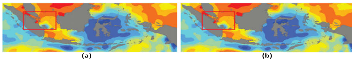
Figure 3-6: Interpolation results from August 24 th 2013, a. IDW; b. Ordinary Krigging
