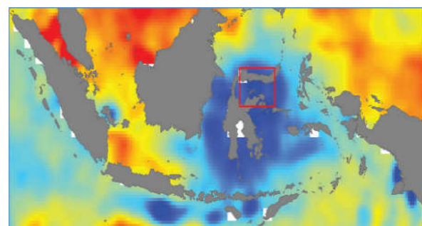
Figure 3-1: Grid data from august 22 nd 2013 before interpolation
