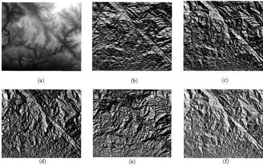
Figure 3-2: DEM SRTM imagery Geumpang area. (a) Before the hillshade processed (b) After done the hillshade 0° (c) After done the hillshade 45° (d) After done the hillshade 90° (e) After done the hillshade 135° (f) After done the overlay
