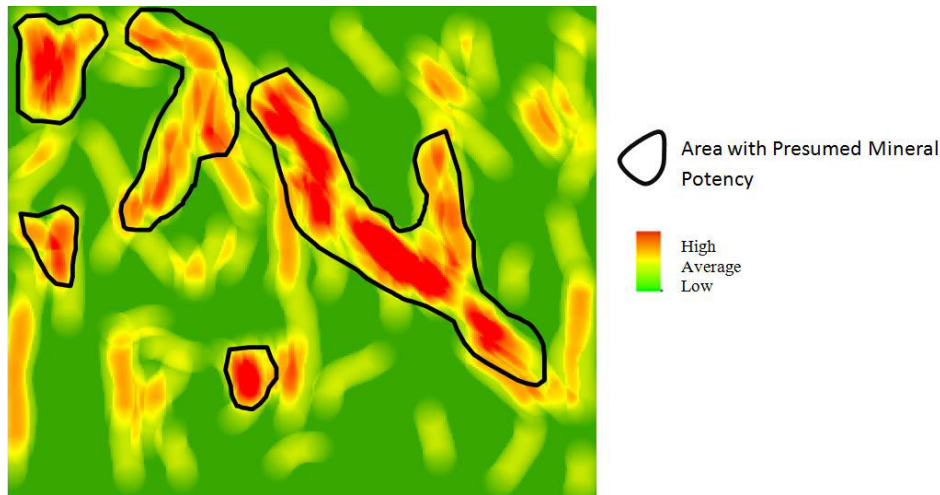
Figure 3-6: Area with presumed mineral potency based on lineament density information
