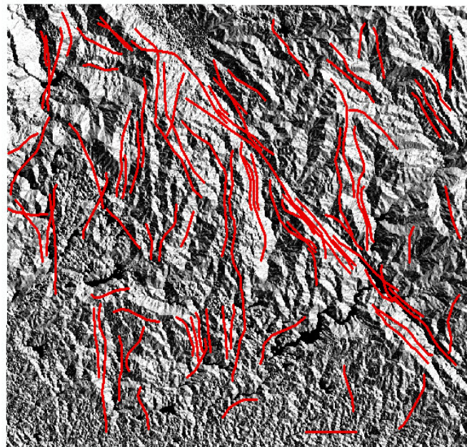
Figure 3-3: The lineament of Geumpang area with the background of DEM SRTM imagery with resolution 30 m
