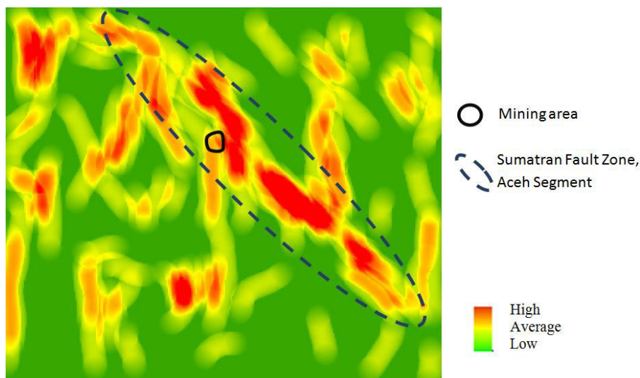
Figure 3-4: The density lineament information, Geumpang area
