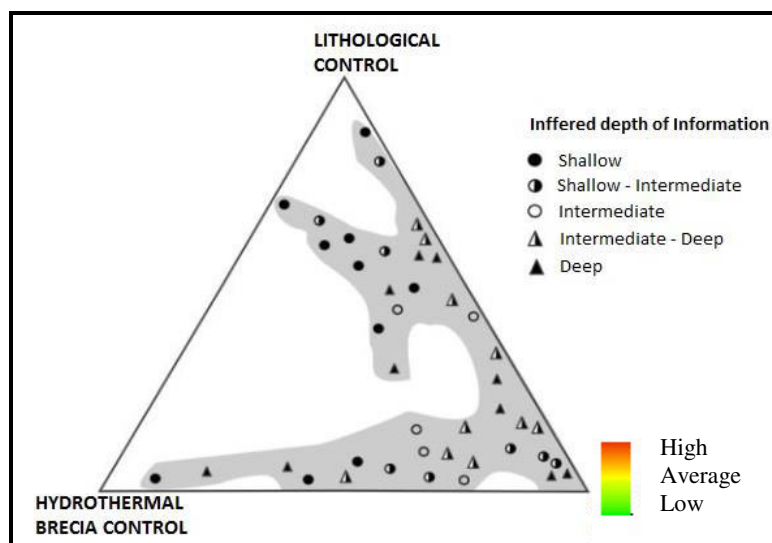
Figure 3-5: Lithostructural concept diagram (Sillitoe, 1999)
