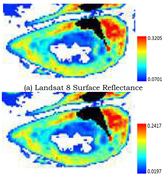
Figure 3-1: Depth Index Distribution
