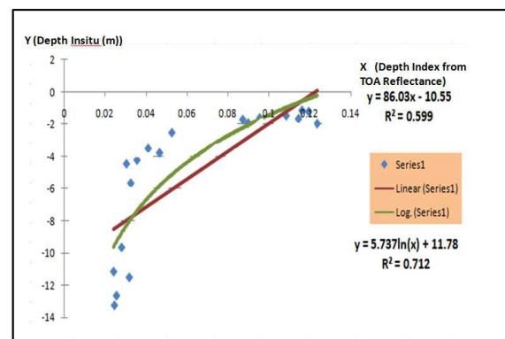
(b) Landsat 8 TOA Reflectance
