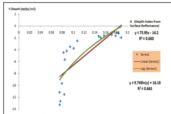
(a) Landsat 8 Surface Reflectance
