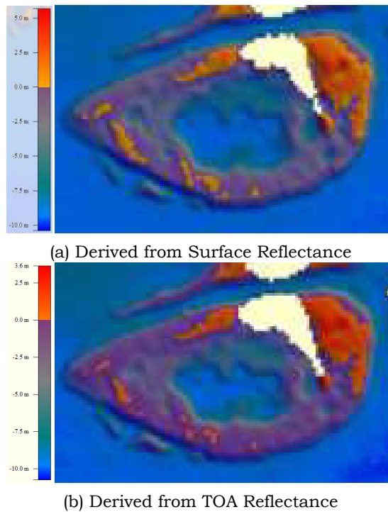
Figure 3-3: Absolute Depth from Landsat 8
