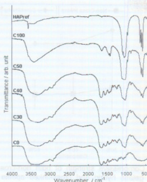
Fig 4. FTIR spectra of cross-linked apatite gelatin hybrid
