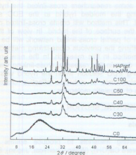
Fig 2. XRD pattern of cross-linked apatite gelatin hybrid
