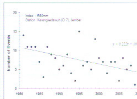
Figure 10. Scatter plot of index R50mm at Station Bangil-left and Karangkedawuh-right
