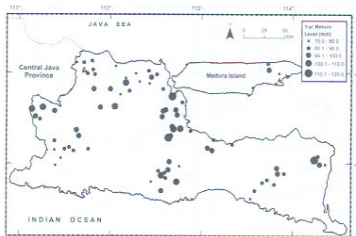
Figure 6. Spatial pattern of threshold for 1-year return period
