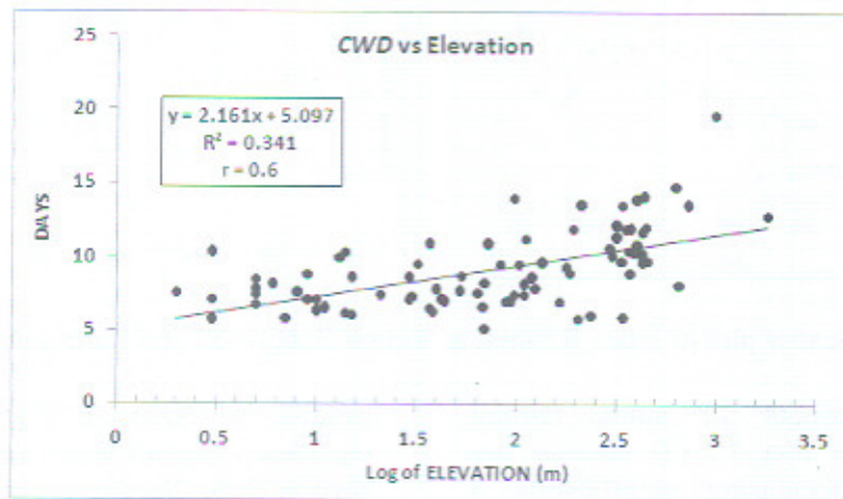
Figure 9. The scatter plot of index CWD versus log of elevation
