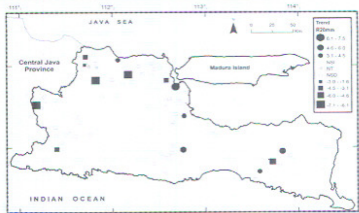
Figure 12. Trend of daily rainfall events exceeding 20 mm. Circle refers to positive trend, square to negative trend. Bold legend corresponds to significant trend. Magnitude is given in “events/decade”. NSI = Not Significant Increasing, NT = No Trend and NSD = Not Significant Decreasing
