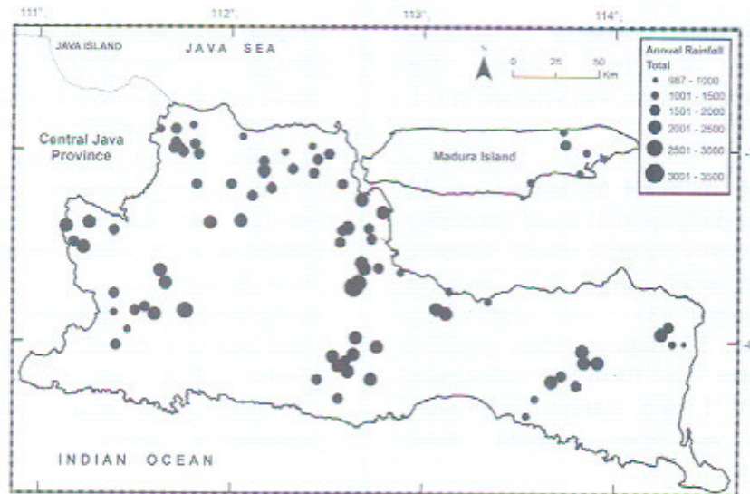
Figure 8. Annual rainfall total over study area
