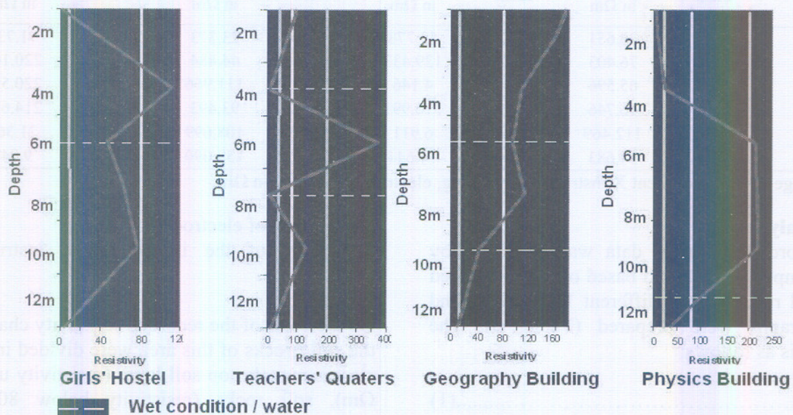
Figure 4. Line graphs showing the electrical resistivity structure at different depths of the VES points
