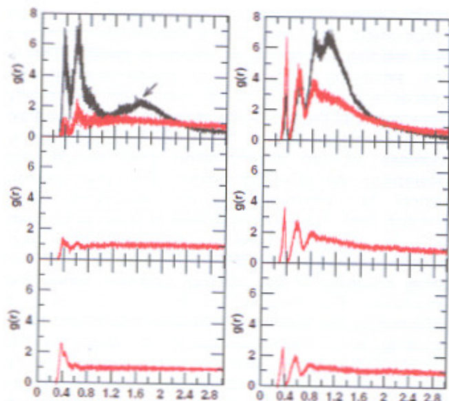
Fig 2. Radial distribution function (RDF) for: cation-cation (left), phosphor-cation (right); from top to bottom: 0.14 M Na + , 0.50 M Na + , and 1.03 M Na + . The g(r) results using reaction field are shown by black curves and using PME red curves. Artifacts at cutoff radius are depicted by black arrows
