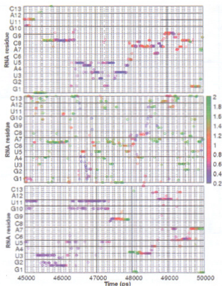
Fig 5. 3D description of minimum distance of ions around RNA in 0.1 M Na + , 1.0 M Na + , and 0.1 M Mg 2+ (from top to bottom). The x-axis corresponds to 45-50 ns simulation time; the y-axis to all electronegative atoms of RNA residues; the color of circle to the minimum distance between an ion and an electronegative atoms. Only one atom is shown
