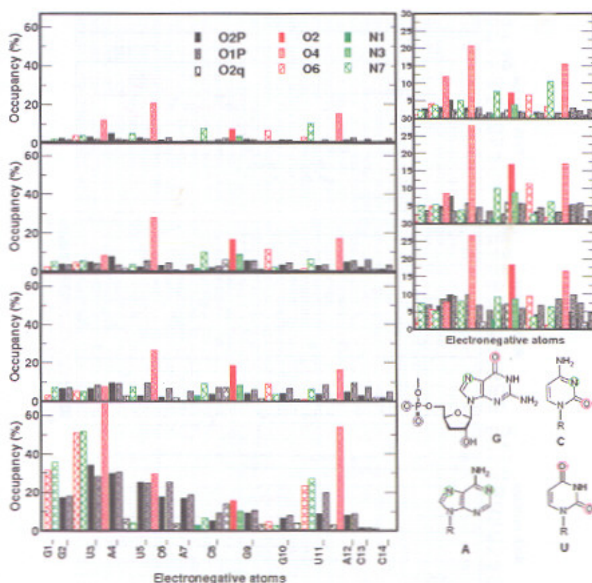
Fig 4. Averaged occupancy of 0.1 M Na + , 0.5 M Na + , and 1.0 M Na + , and 0.1 M Mg 2+ (from top to bottom) around electronegative atoms of uCACGg hairpin. The symbols for the electronegative atoms are represented (top). To compare ion occupancy of Na + with different concentration, zooms of ion occupancies are provided in the right side. To highlight the certain electronegative atoms, these atoms are showed inside circles in the right bottom
