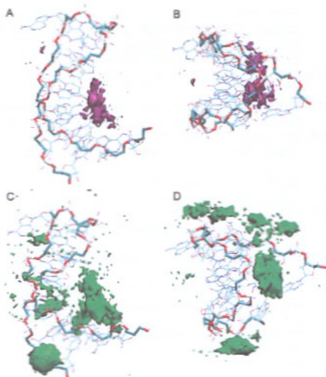
Fig 6. Spatial distribution function (SDF) of \text{Na}^+ (violet) and \text{Mg}^{2+} (green) around averaged structure of uCACGg hairpin. To highlight the preferential presence of the ions, the backbone atoms have been displayed thicker than the rest atoms of the hairpin, and certain residues are signed. For the best display, the SDFs of ions are illustrated in top view (B and D) and side view (A, and C). The isosurfaces correspond to g(r, \omega)=60
