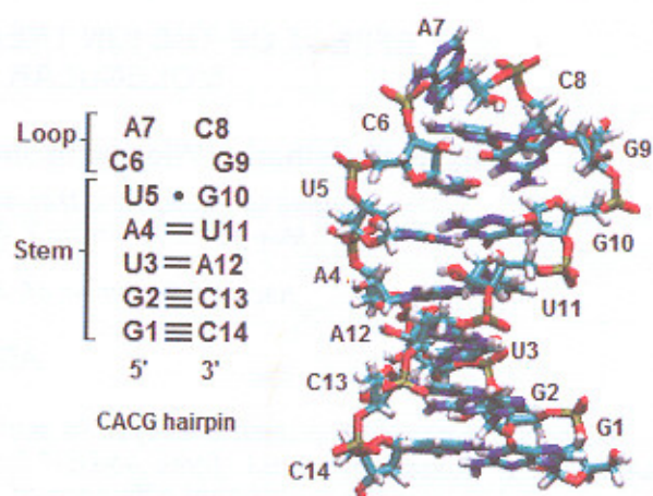
Fig 1. The 14-mer uCACGg hairpin which consists of a stem and a loop region with numbering. (A) Secondary and (B) tertiary structure. The lines which connect two bases represent the hydrogen bonds between Watson-Crick base-pairs, and the black point wobble base-pair.
