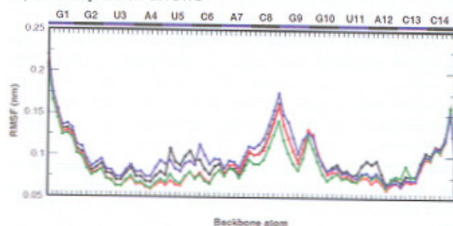
Fig 3. RMSF of backbone atoms and O2P/C14 relative to their average positions after fitting to all atoms for uCACGg hairpin at different concentration of Na + and Mg 2+ . The black, red, green and blue lines show 0.14 M Na + , 0.50 M Na + , 1.03 M Na + 0.08 M Mg 2+
