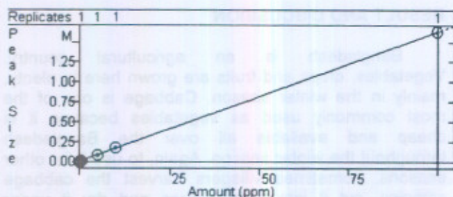
Fig 2. Calibration curve of nonadecane standard (Column: VF-5 (l. 30 m, i.d. 0.25, film thickness 0.25 \mu m); delay: 5 min; Temperature Program: 50°C(1)→200 °C (8 °C/min) →300°C (10 °C/min); Injector Temperature: 250 °C; Split: 20%; Injection volume: 1 \mu L; Carrier gas: He; Flow rate: 1mL/min.)
