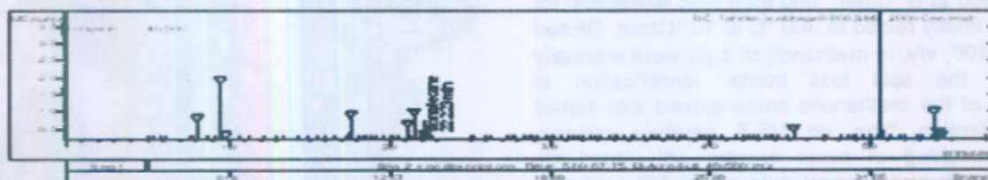
Fig 5. TIC Chromatogram of the cabbage samples from the district of Manikgonj
