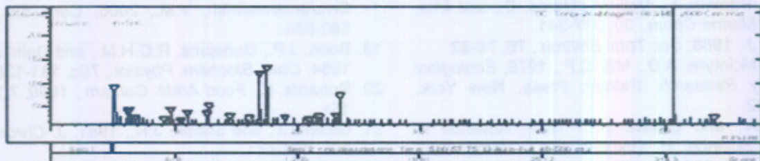
Fig 8. TIC Chromatogram of the blank samples
