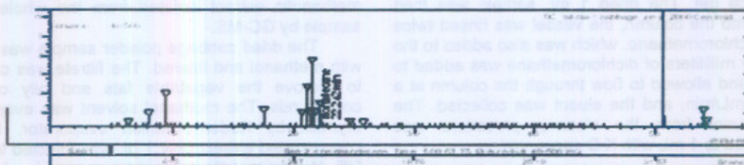
Fig 3. TIC Chromatogram of the cabbage samples from the Talola, Dhaka (Column: VF-5 (l. 30m, i.d. 0.25, film thickness 0.25 \mu m); delay: 5 min; Temperature Program: 50 °C(1)→ 200°C (8 °C/min) →300 °C (10 °C/min); Injector Temperature: 250 °C; Split: 20%; Injection volume: 1 \mu L; Carrier gas: He; Flow rate: 1mL/min.)
