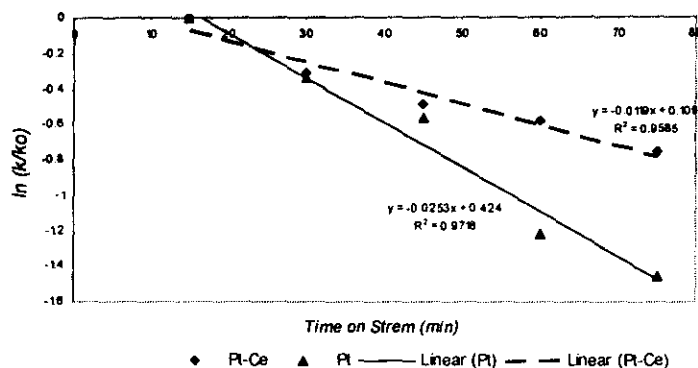
Fig 2. Ln relative rate constants ( k/k_0 ) for reaction on the Pt-Ce/zeolite and Pt/zeolite catalysts at 350 °C vs Time on Stream
