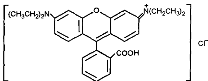
Fig 1. Structure of rhodamin-B
