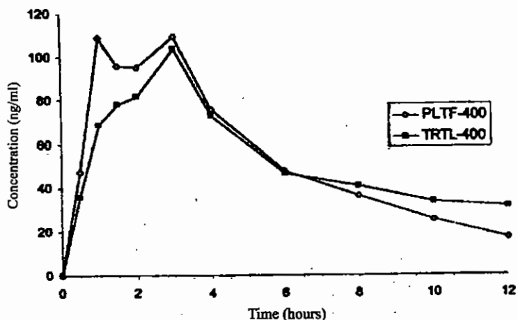
Figure 1. Plasma level-time courses of pentoxyphylline following administration of each product (mean in 12 subjects)
