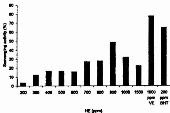
Figure 1. Effects of hexane extract (HE) at different concentrations on scavenging 1,1- diphenyl-2-picrylhydrazyl (DPPH) free radical (2 mM)
