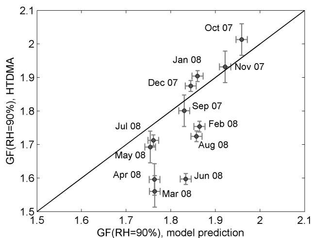
Figure 4. Comparison of calculated monthly growth factors using the hygroscopic model and the sampled H-TDMA measurements at RH = 90 % for aerosol particles in the size range of 80–120 nm, from September 2007 to August 2008.
