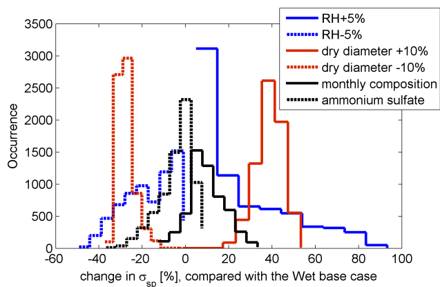
Figure 10. Sensitivity of the hourly calculated \sigma_{sp} to RH, aerosol dry size and chemical composition as compared with the Wet base case (see Table 2).
