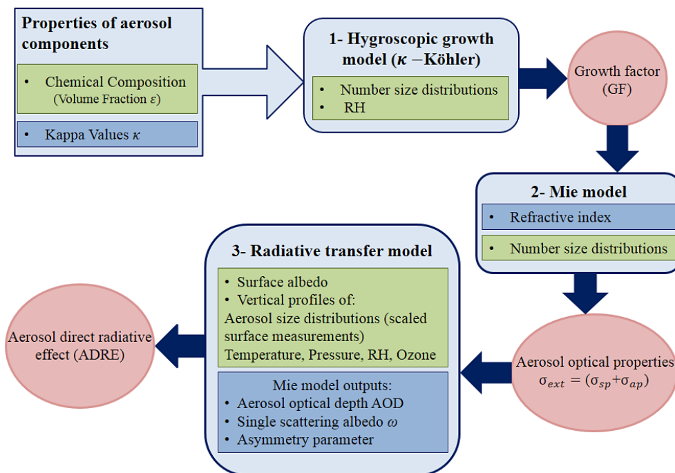
Figure 2. Scheme of the models and their required input, starting with the hygroscopic growth model and ending with the radiative transfer model to calculate the ADRE. The light blue boxes refer to the different model calculations, the green boxes to experimental input data, the dark blue boxes to additional input data (e.g., from literature), and the red circles denote model output.
