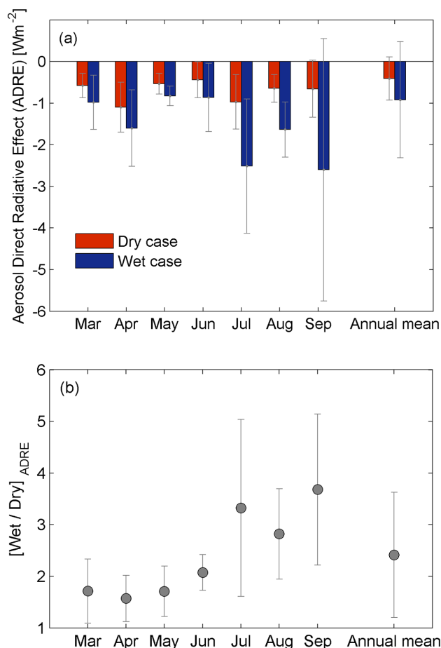
Figure 12. (a) Monthly and annual averaged ADRE for the Dry and Wet cases (see Table 2) at the Zeppelin station for 2008. For the months not shown the ADRE is assumed to be zero due to lack of sunlight. (b) The ratio between Wet and Dry ADRE. The error bars indicate the standard deviations.
