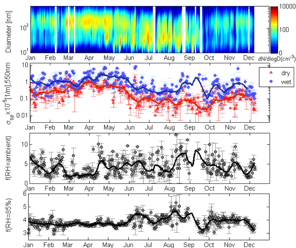
Figure 9. (a) Number size distributions measured at the Zeppelin station for year 2008. (b) The calculated daily mean scattering coefficients for the Dry and Wet cases (see Table 2). (c) The calculated daily mean enhancement factors f (ambient RH) for the Wet case. (d) The four calculated daily mean enhancement factors f (RH = 85 %). In all figures the error bars indicate standard deviations. Note that the scale is different in (c) and Fig. 10d.
