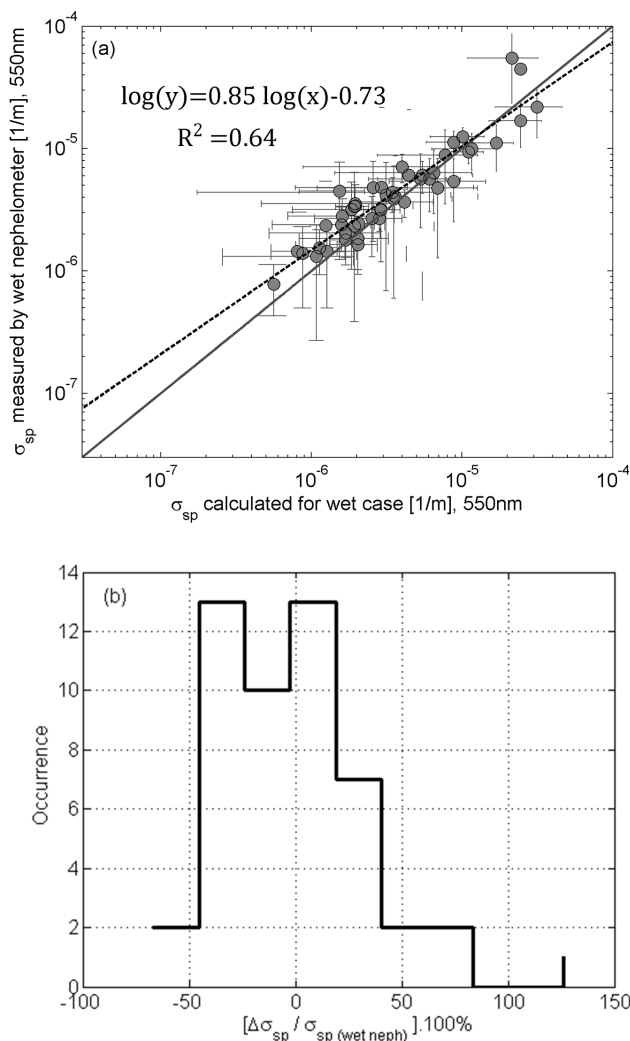
Figure 6. (a) Correlation between modeled and measured daily mean wet \sigma_{sp} (550 nm) at the ambient RH for the campaign (15 July–12 October 2008). The error bars indicate the standard deviations of the daily averages. (b) Histogram of the deviation of modeled scattering coefficient from measurements in percentage (%).
