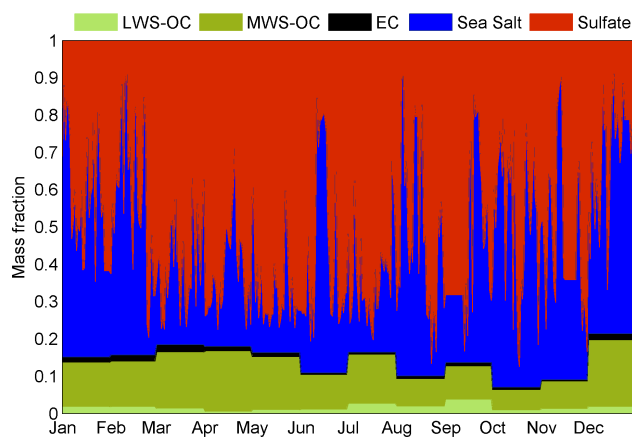
Figure 3. The averaged chemical composition for year 2008 at the Zeppelin station based on filter measurements, on a daily basis for inorganics (sea salt and sulfate) and monthly basis for organics (LWS-OC, MWS-OC, EC).
