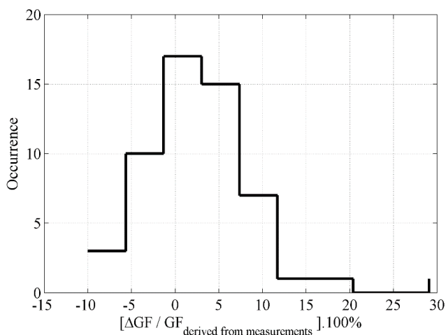
Figure 7. Histogram of modeled growth factor deviations from values derived from the humidified nephelometer measurements in percentage (%) during the campaign.
