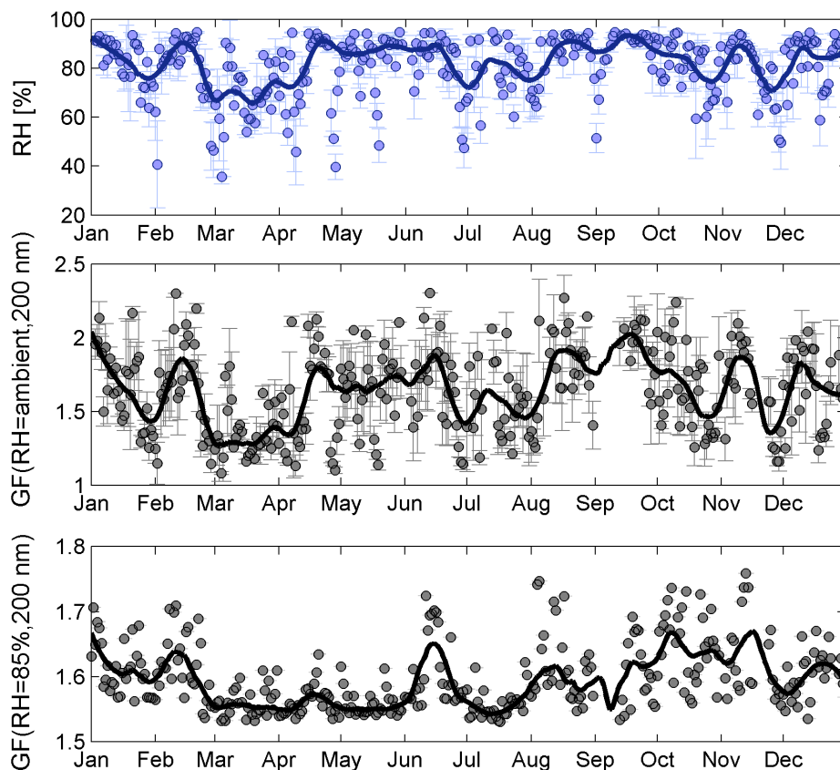
Figure 8. (a) Daily mean relative humidity (%) measured at the Zeppelin station for year 2008. (b) The calculated daily mean GFs assuming ambient RH for an initial size of 200 nm. (c) The calculated daily mean GFs at RH = 85 % for initial size of 200 nm. In Fig. 9a and b the error bars indicate standard deviations.
