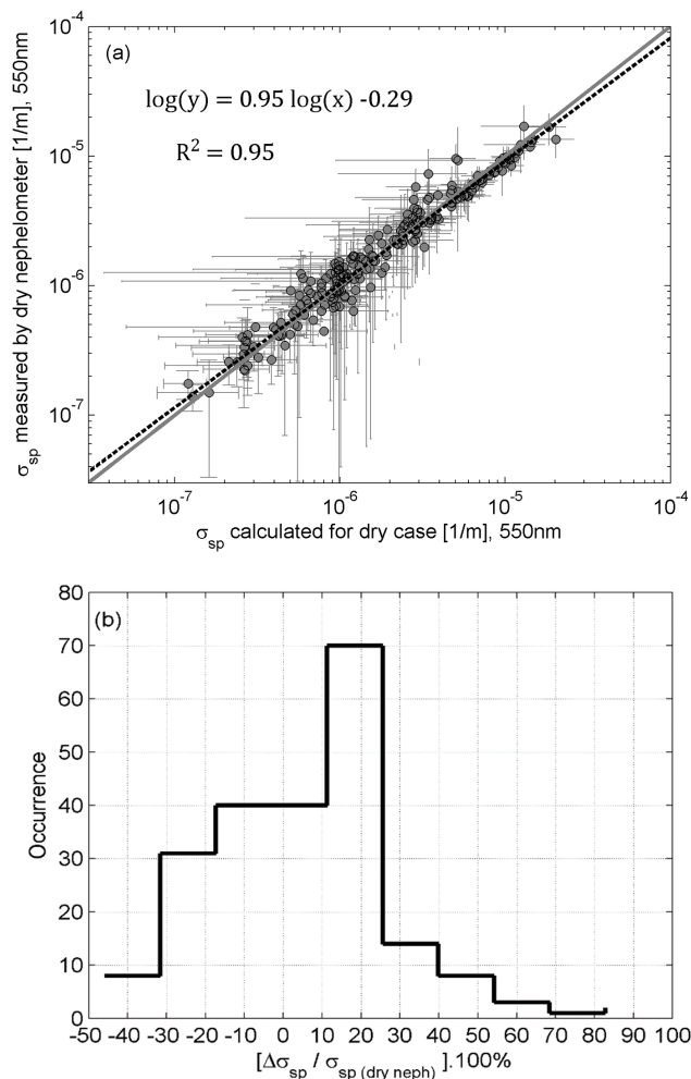
Figure 5. (a) Correlation between modeled and measured daily mean dry \sigma_{sp} (550 nm) for the year 2008. The error bars indicate the standard deviations of the daily averages. (b) Histogram of the deviation of the modeled scattering coefficient from measurements in percentage (%).
