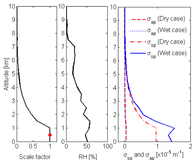
Figure 11. Vertical profile of (a) scale factor for particle number size distributions, the red point shows the level of the station. (b) Ambient RH measured by soundings. (c) \sigma_{sp} and \sigma_{ap} m^{-1} , modeled for the Dry and Wet cases for 11 April 2008 at the Zeppelin station.
