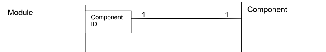
Figure 13 Weak Entity as a qualified association.
