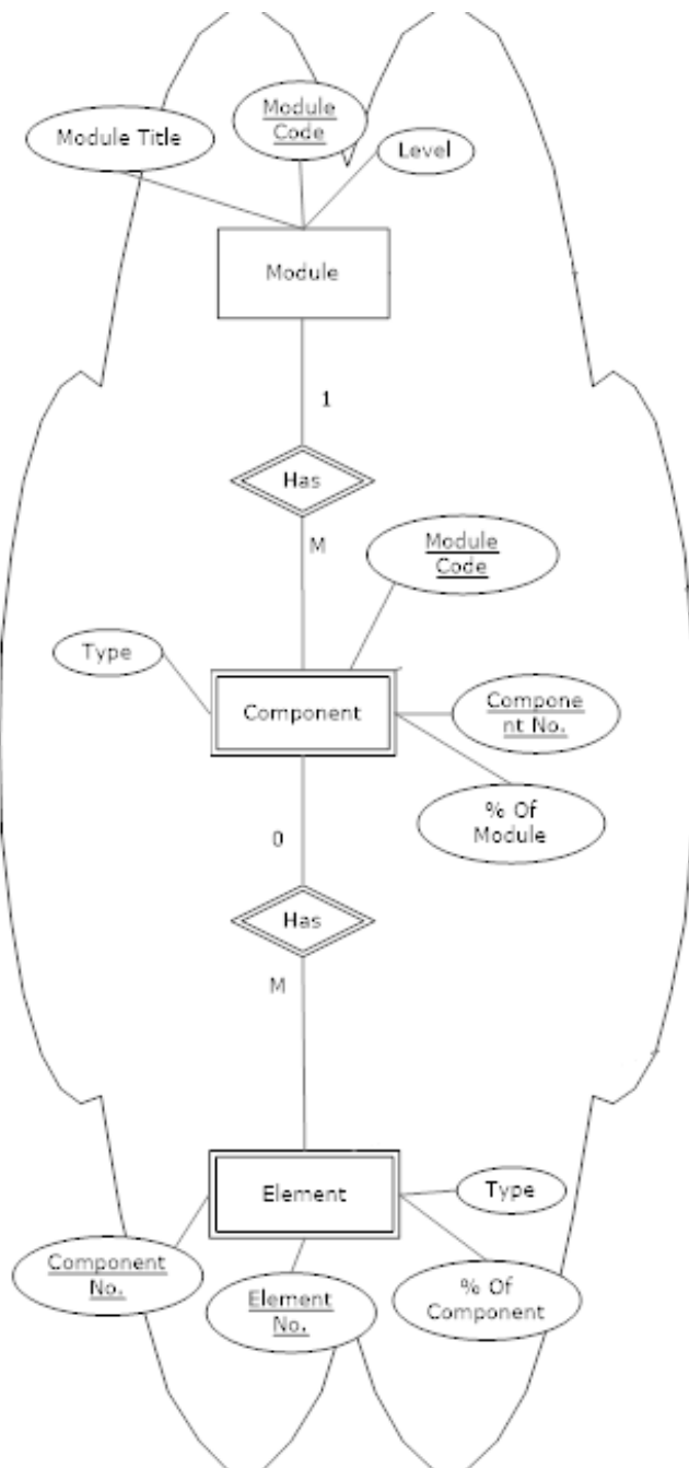
Figure 8 ER notation for aggregation (Module may have many components, components may have many elements)
