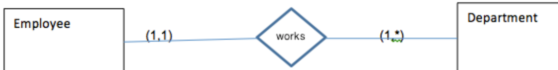
Figure 6 Elmasri and Navathe notation – Look here notation.
