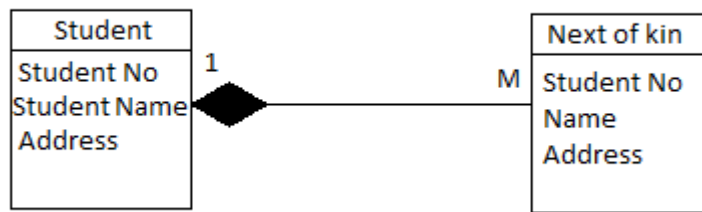
Figure 10 Possible notation for Weak Entity
