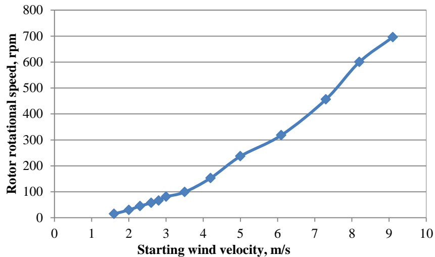
Fig. 14. Experimental maximum rotational speeds versus starting wind velocities.
