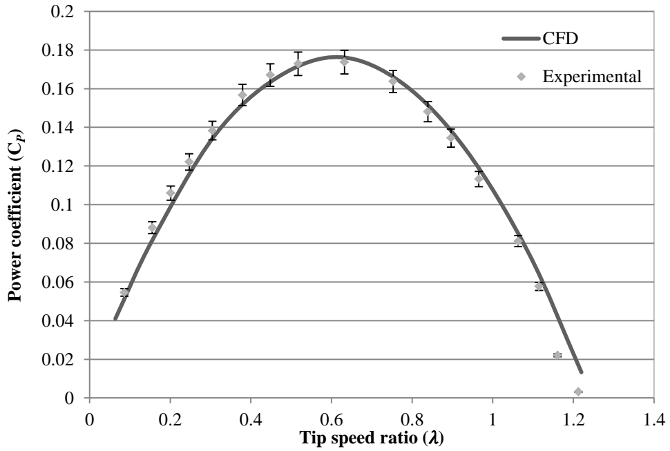
Fig. 12. Comparison of power coefficients from tests and CFD simulations at U = 8.2\text{m/s}
