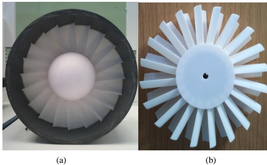
Fig. 2. The wind turbine prototype produced by rapid manufacturing technology: (a) the stator with 20 guide vanes inside a cylinder flow chamber; (b) the rotor with 20 blades
