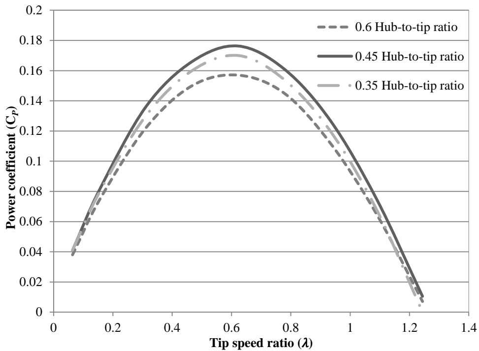
Fig. 13. Comparison of power coefficients under three hub-to-tip ratios at U = 8.2\text{m/s}
