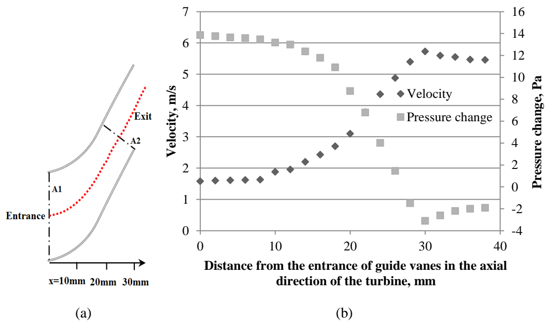
Fig. 8. Distribution of the flow velocity and the pressure change along the centre line of the flow passage: (a) schematic view of the flow passage between two guide vanes; (b) flow velocity and pressure change along the centre line of the flow passage at r = 100\text{mm}
