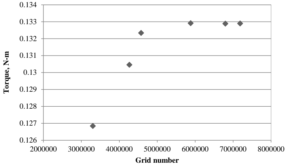
Fig. 6. Torque values under different grid numbers
