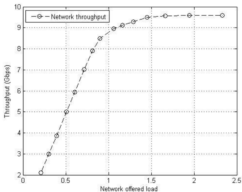
Figure 4 Network throughput
