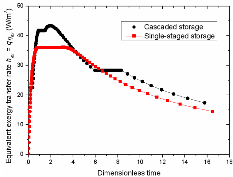
Fig. 4. A comparison of the equivalent Exergy Flow h_{ex}
