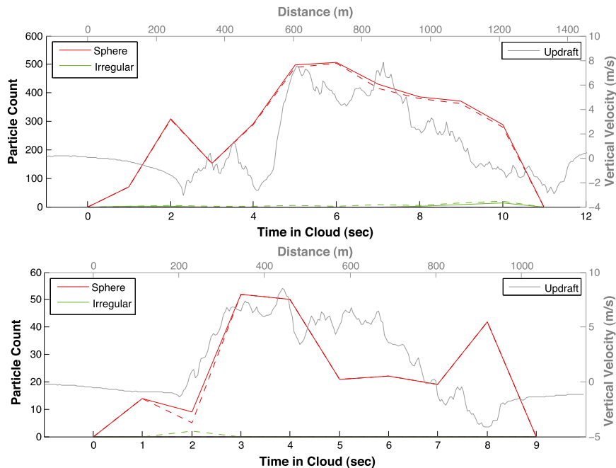
FIG. 6. Warm cloud passes at +7^{\circ}\text{C} from (a) 11 Jul 2011, starting at 1810:49 UTC; and (b) 12 Jul 2011, starting at 1844:33 UTC, within 500 m of the cloud top. Original (dashed lines) and corrected (solid lines) particle counts for sphere and irregular particles detected by the SID-2H (left axis) and updraft vertical velocity (gray line, right axis) as measured during the cloud pass over time (bottom axis) and distance in cloud (top axis).
