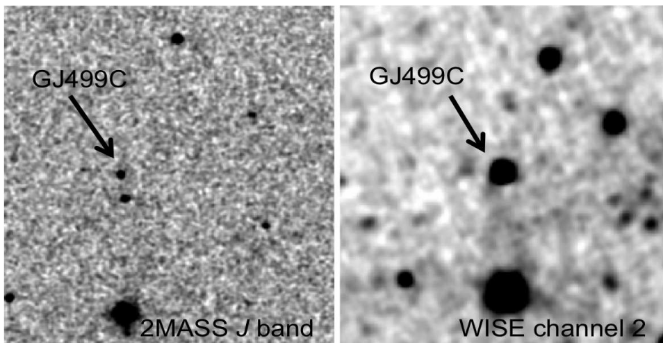
Figure 4. A 5 arcmin \times 5 arcmin finder chart for the GJ499C dwarf. On the left panel is the J band image and on the right one the W2 band. North is up and East is left.
