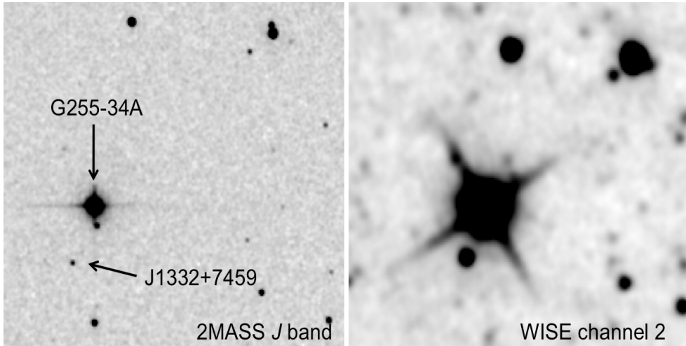
Figure 3. A 4.5 arcmin \times 4.5 arcmin finder chart for the system G255-34AB. On the left panel is the J band image and on the right one the W2 band. North is up and East is left.
