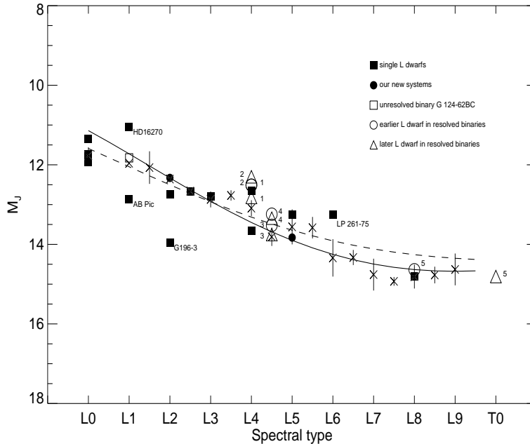
Figure 5. Spectral type vs M_J for the L dwarf + MS star systems in Table 6. The filled squares are those systems with only one L dwarf, the filled circles are the two new systems presented in this paper. The systems in which there are two unresolved L dwarfs and a MS star are represented by two symbols, an open circle showing the earlier of the two UCDs and an open triangle showing the later type UCD. The dashed line shows the polynomial fit from Faherty et al. (2012) and the solid one the fit from Marocco et al. (2010). The crosses represent the mean 2MASS M_J for each spectral type (Dupuy & Liu et al. 2012). The numbers represent the following systems: (1) GJ 564ABC; (2) HD2057ABC; (3) GI 417ABCD; (4) GJ 1001ABC; (5) GI 337ABCD.
