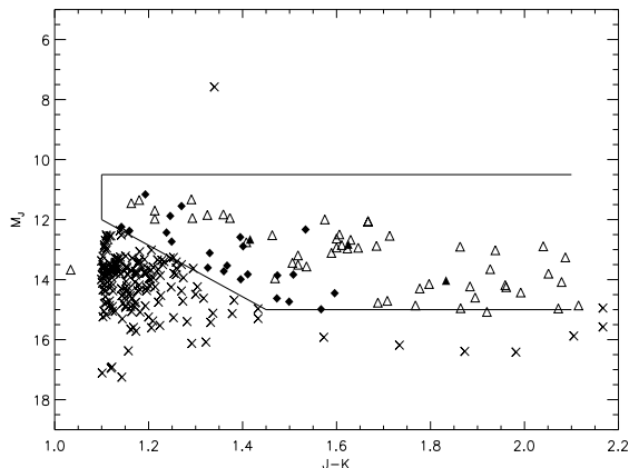
Figure 1. M_J versus J - K colour-magnitude diagrams. The UCDs from the candidate pairs are shown as crosses. Inside the selection box, the filled triangles are the three known L dwarfs that turn up in our sample as possible binaries, the filled diamonds are UCDs candidates not confirmed and not in the dwarfarchive.org. The open triangles represent other UCDs with known parallax measurements from Dwarf Archives and are displayed for comparison purposes only.
