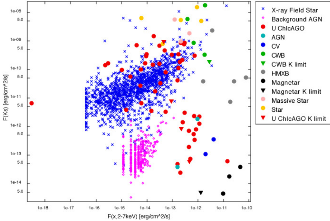
Figure 7. Observed K_s -band flux ( F_{K_s} ) vs absorbed 2–7 keV X-ray flux ( F_{x,2-7\text{keV}} ) of unidentified ChlcAGO sources (“U ChlcAGO:” red points) and identified ChlcAGO and archival sources. Triangular data points represent those sources that only have upper limits on their K_s -band fluxes. The Chandra Orion Ultradeep Project sources (blue crosses) and the XBootes Survey sources (magenta diamonds), which are predominantly PMS stars and background AGN, respectively, are also included. The lone red data point on the far left of the diagram (ChI J154557–5443_3) should be treated as a X-ray flux upper limit as Chandra detected very few hard X-ray counts ( > 2 keV) from this source. This plot is based upon Figure 5 of Gelfand & Gaensler (2007).
