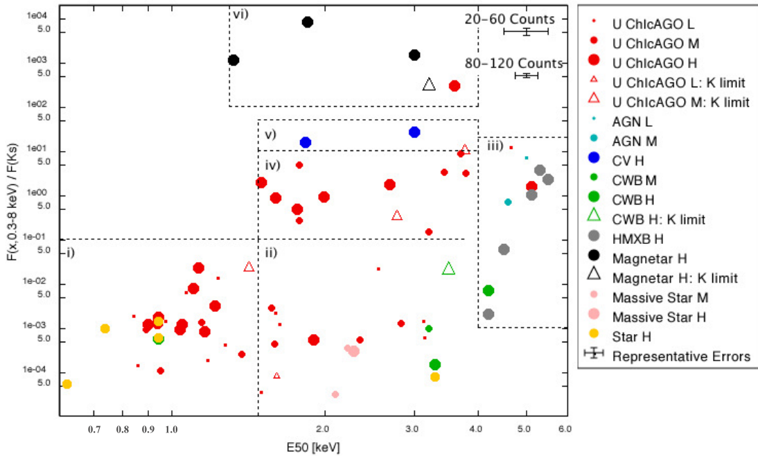
Figure 8. Observed X-ray-to- K_s -band flux ratio ( F_{x,0.3-8\text{keV}}/F_{K_s} ) vs median energy ( E_{50} keV) of unidentified ChlcAGO sources and the identified ChlcAGO and AGPS sources. The different sizes of data points represent whether a given source has a low count-rate (L as listed in the legend), medium count-rate (M) or a high count-rate (H). The unidentified ChlcAGO sources (“U ChlcAGO”) are represented by red data points and the identified ChlcAGO and archival sources are in other colors. The triangles represent those sources that only have upper limits on their K_s -band fluxes, implying lower limits on their F_x/F_{K_s} ratios. The representative error bars demonstrate the sizes of errors expected from a 20–60 count X-ray source or a 80–120 count X-ray source. This plot has been divided into 6 regions, indicated by the dashed lines and Roman numerals, in order to further explore the source populations (see Section 4.2).
