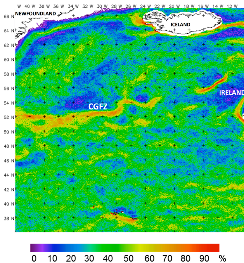
Figure 1.1 Front mapping via EO Remote Sensing. Example imagery: seasonal front frequency map, N. Atlantic (percent time a front detected in each 1km pixel during spring, March-May). Regions of frequent mesoscale frontal activity along the North Atlantic Current are highlighted, including that associated with the Charlie Gibbs Fracture Zone. Useful as part of a suite of tools for locating priority conservation areas through identifying potential biophysical hotspots of significance to marine vertebrates, and their dynamics through time. Derived from merged microwave and infrared SST data, 2006-2011. Reproduced, with permission, from Miller et al. (2013).
