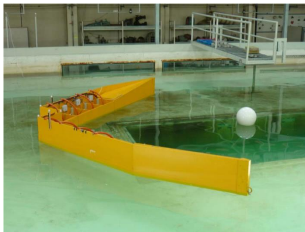
Figure 4. The WaveCat, a novel overtopping type of WEC (Fernandez et al., 2012).
