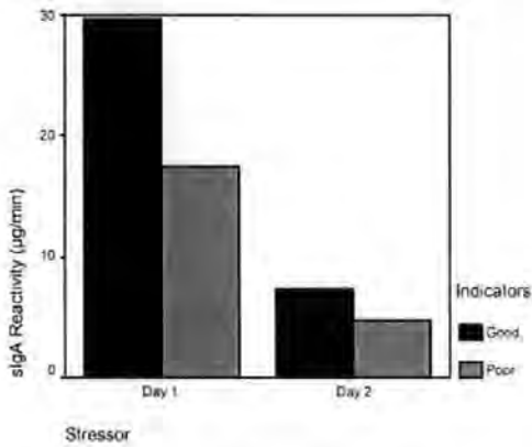
Figure 6.16 S-IgA Reactivity to Acute Stress in Volunteers With Good or Poor Indicators of ill-health
