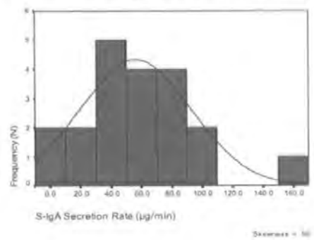
Post-stress S-IgA Secretion rate
