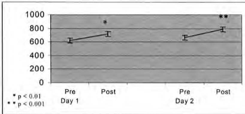
Figure 6.12 Pre and Post Saliva Volume (and SEM) on Days One and Two
