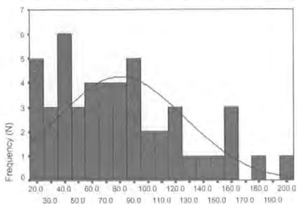
Day One Pre-stress S-IgA Secretion Rate
