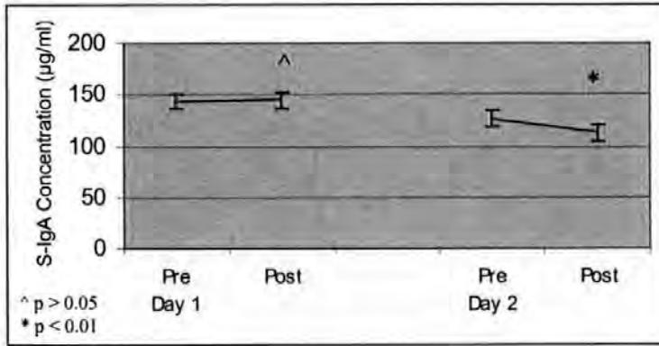
Figure 6.1 S-IgA Reactivity to Acute Stress (and S.E.M)
