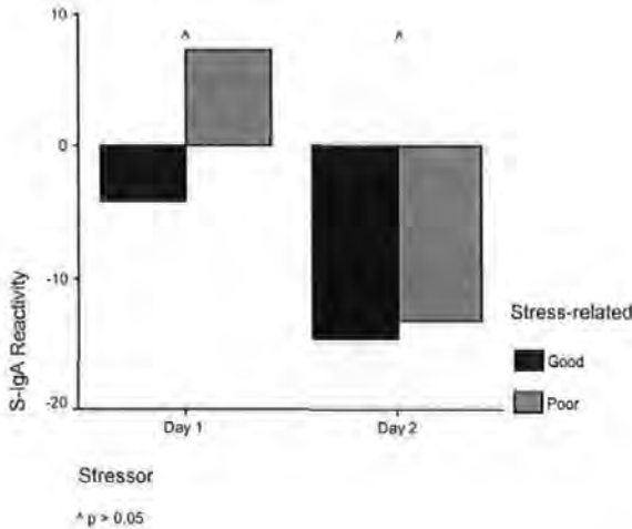
Figure 6.3 S-IgA Reactivity in Volunteers with Good and Poor Stress-related Complaints
