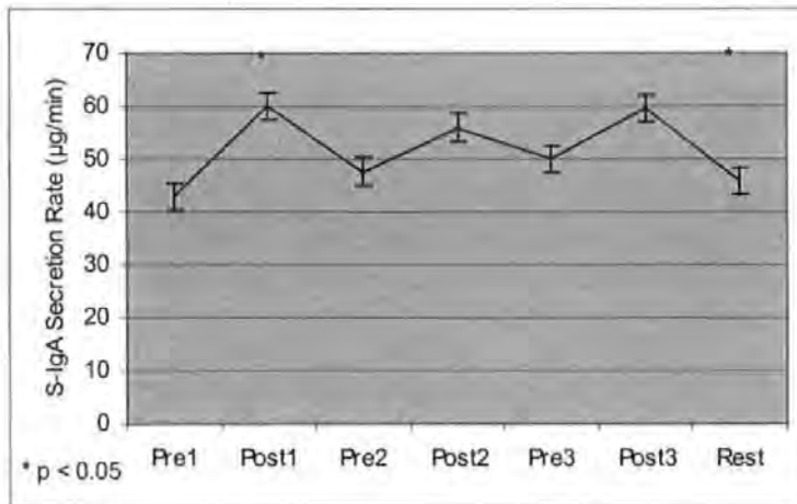
Figure 7.2 S-IgA Reactivity (and SEM) to Cumulative Acute Stress
