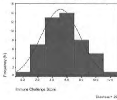
Immune Challenge Complaints
