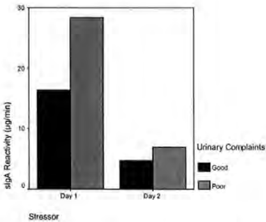
Figure 6.21 S-IgA Reactivity to Acute Stress in Volunteers With Good or Poor Urinary-tract Complaints
