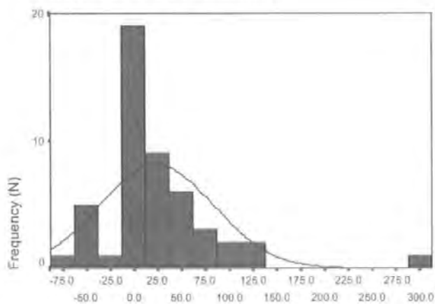
Day One S-IgA Reactivity
