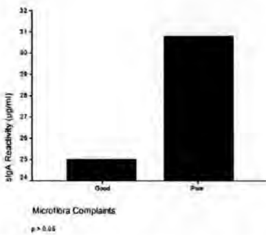
Figure 5.10 S-IgA Reactivity in Volunteers with Good and Poor Microflora Complaints
