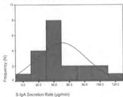
Pre-stress S-IgA Secretion Rate
