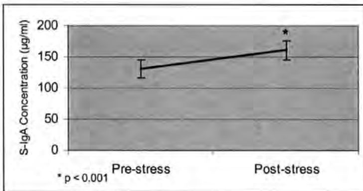
Figure 5.1 S-IgA Reactivity to Acute Stress (and S.E.M)
