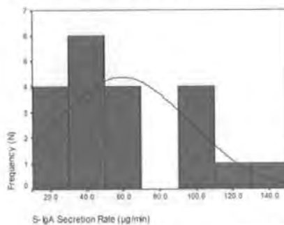
Post-stress S-IgA Secretion rate
