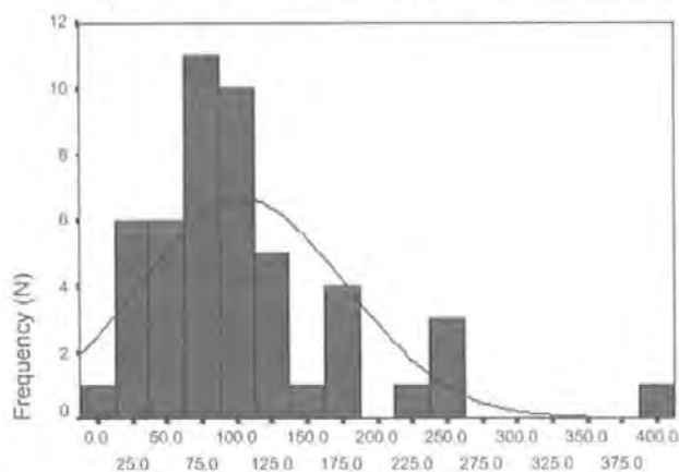
Day Two Post-stress S-IgA Secretion Rate
