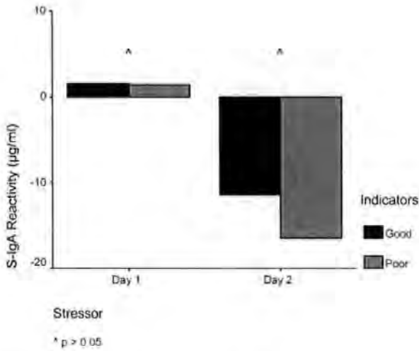
Figure 6.4 S-IgA Reactivity in Volunteers with Good and Poor Indicators of Ill-health
