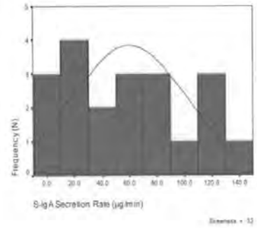
Post-stress S-IgA Secretion Rate
