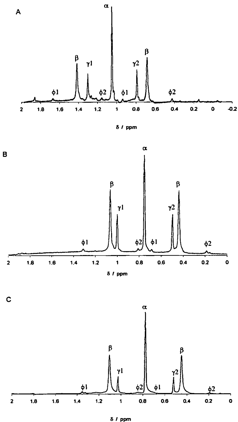
Figure 2-6 ^1\text{H} NMR spectrum of ^{13}\text{CH}_3\text{HgI} (1 mg/ml) and ^{199}\text{Hg} enriched \text{CH}_3\text{HgCl} (2 mg/ml) in 50:50 \text{D}_2\text{O}/\text{CH}_3\text{OD} v/v, 0.01% 2-mercaptoethanol: A, prior to injection onto the HPLC column; B, the post-column eluent fraction containing the methylmercury species; and C, the pre injection mixture after solvent evaporation by gaseous \text{N}_2 . KI was added to the samples prior to analysis by ^1\text{H} NMR spectroscopy.
