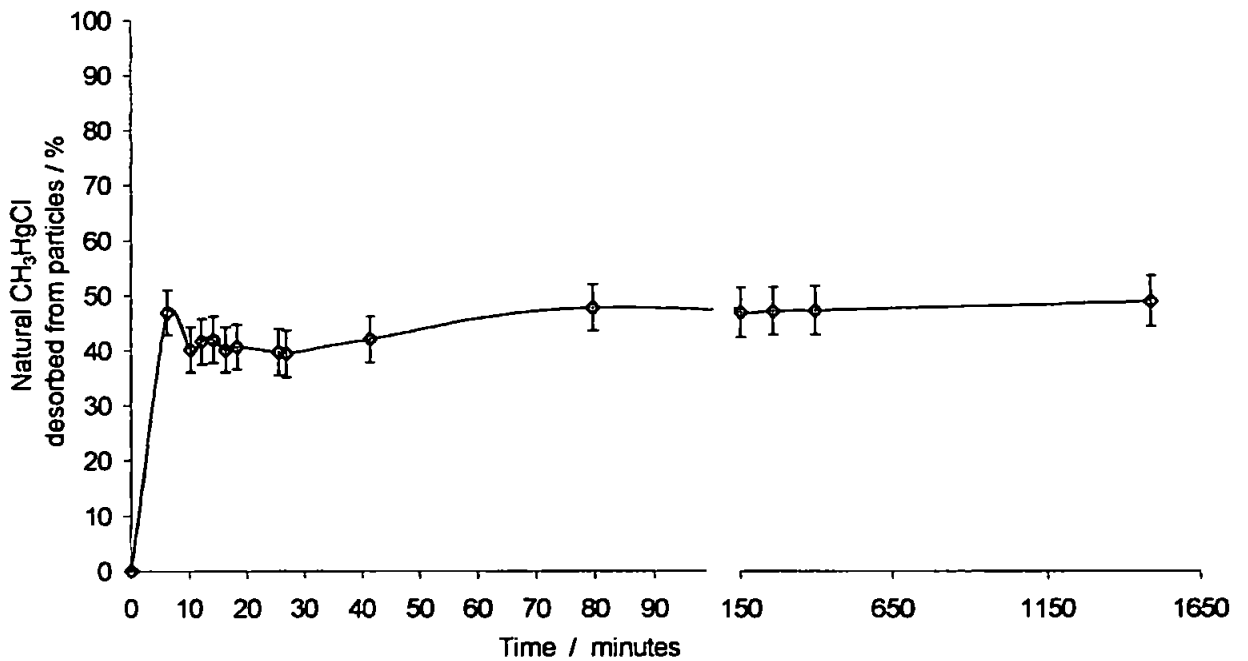
Figure 4-5 The amount of; A, 199 Hg enriched methylmercurychloride remaining in solution; B, of particulate bound natural isotopic methylmercurychloride desorbed during the IDMS determination of methylmercury in DORM-2. Uncertainty bars are the expanded uncertainty ( k = 4.3 ).
