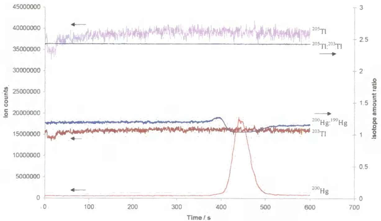
Figure 5-5 The measured, by HPLC-CV-MC-ICP-MS, ^{200}\text{Hg}:^{199}\text{Hg} and ^{205}\text{Tl}:^{203}\text{Tl} isotope amount ratios and ^{200}\text{Hg} signal monitored for a 100\mu\text{l} injection of methylmercury chloride, 1\mu\text{g g}^{-1} as Hg. A, with the CV generation inlet tube unbent; B, with the CV generation inlet tube formed into a 'U' shape.
