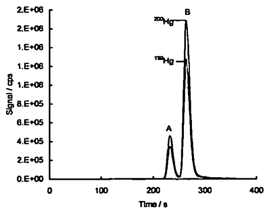
Figure 3. HPLC-ICP-MS Chromatogram of: A, inorganic mercury (210 ng) and; B, methylmercurychloride (900 ng), obtained by monitoring the 199 Hg and 200 Hg isotopes.
