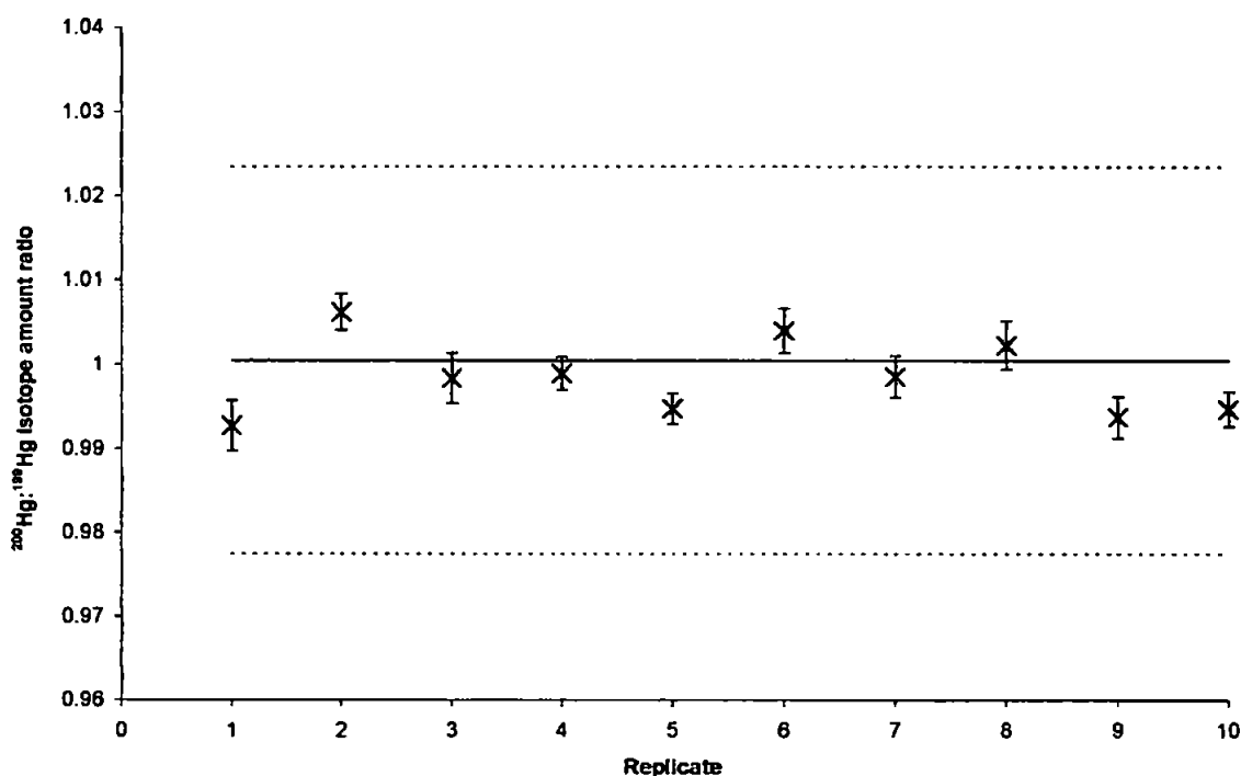
Figure 5-6 The ^{200}\text{Hg}:^{199}\text{Hg} isotope amount ratios, calculated by the pseudo-steady-state approach, from a 500\mu\text{l} injection of a blend of natural isotopic abundance and ^{199}\text{Hg} enriched methylmercurychloride, 30\text{ ng g}^{-1} as Hg. The error bars represent the expanded uncertainty ( k = 2 ). The solid horizontal line is the value calculated from the masses and mass fractions of the individual solutions used to prepare the blend, with the dashed lines representing the upper and lower limits of the expanded uncertainty ( k = 2 ).
