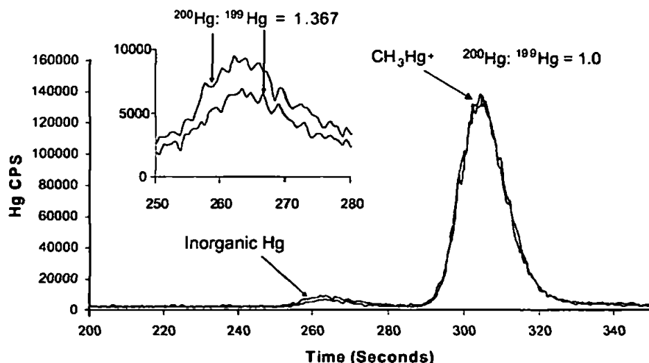
Fig. 4 HPLC-ICP-MS chromatogram of an equilibration sample with, inset, the co-extracted inorganic Hg from DORM-2 with a natural abundance 200 Hg: 199 Hg isotope amount ratio, indicating that the 199 Hg enriched spike material was stable during the time period of the experiment.
