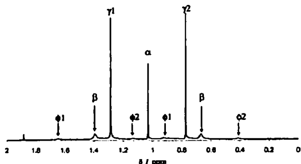
Fig. 2 ^1\text{H} NMR spectrum of ^{13}\text{CH}_3\text{HgI} ( 4.8 \text{ mg ml}^{-1} ) and ^{199}\text{Hg} enriched \text{CH}_3\text{HgI} ( 2 \text{ mg ml}^{-1} ) in \text{CD}_2\text{OD} . The ^1\text{H} - ^{13}\text{C} doublet, marked \gamma_1 and \gamma_2 , arises from the ^{13}\text{CH}_3\text{HgI} : each of these doublets has two associated ^1\text{H} - ^{199}\text{Hg} satellites marked \phi_1 and \phi_2 , respectively. The ^{199}\text{Hg} enriched \text{CH}_3\text{HgI} molecule gives three signals in the spectrum, the main proton signal, \alpha , and two ^1\text{H} - ^{199}\text{Hg} satellites, marked \beta .
