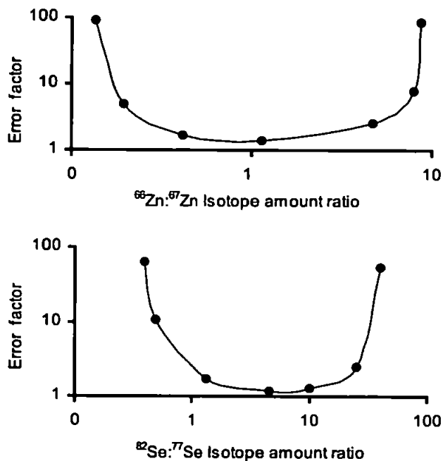
Figure 2. Error propagation plots for the ^{66}\text{Zn}: ^{67}\text{Zn} and ^{82}\text{Se}: ^{77}\text{Se} isotope amount ratios. These plots show the theoretical optimum spiking ratio needed to achieve the best precision for the ratio measurements.
