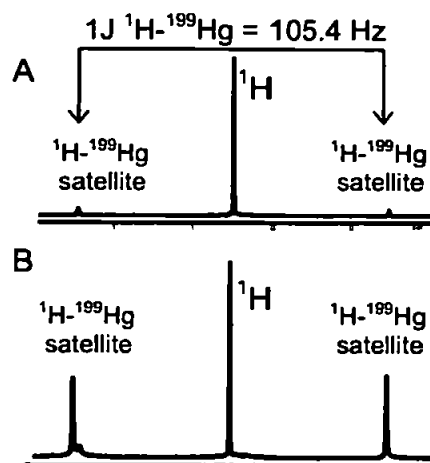
Figure 1. 1 H NMR spectra of A; 1 mg/ml natural isotopic abundance CH 3 HgCl and B; 1 mg/mL 199 Hg enriched CH 3 HgCl. The 199 Hg enrichment can be clearly seen by the increase in the peak areas of the two peaks, which arise from spin-spin coupling between the 1 H and 199 Hg nuclei. Both compounds were dissolved in deuterated methanol, CD 3 OD, for spectral acquisition.
