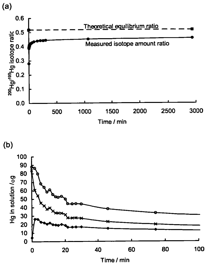
Figure 9. Extraction of inorganic Hg from a sediment certified reference material, which has been spiked with an isotopically enriched analogue. (a) Isotope amount ratio monitored in the liquid phase over the course of the extraction—note that the ratio does not reach the theoretical equilibrium value, indicating that some of the Hg is not easily exchangeable; (b) the extent of adsorption and desorption of Hg, originating from spike and sample, over the course of the extraction procedure.
