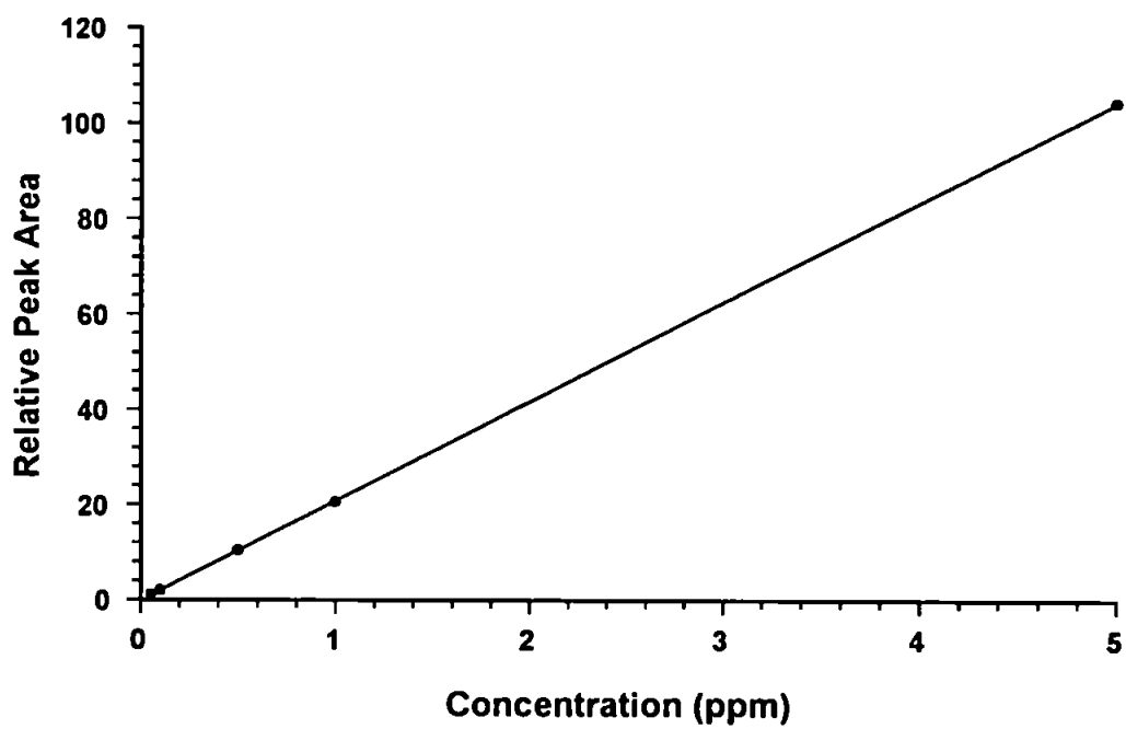
Figure 6.6 Calibration graph for 100 \mu l injections of U(VI) standards
