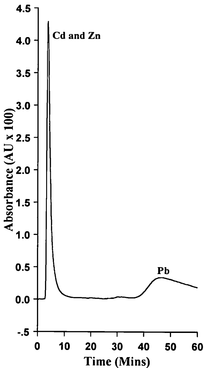
Figure 3.8. 100 \mu\text{l} injection of 10 \mu\text{g ml}^{-1} Zn(II), 20 \mu\text{g ml}^{-1} Cd(II) and 20 \mu\text{g ml}^{-1} Pb(II) using the PP column. The eluent was 0.5 \text{ mol dm}^{-3} \text{KNO}_3 and 0.05 \text{ mol dm}^{-3} lactic acid, adjusted to pH 4 with dilute ammonia. Detection was with PAR at 490 nm.
