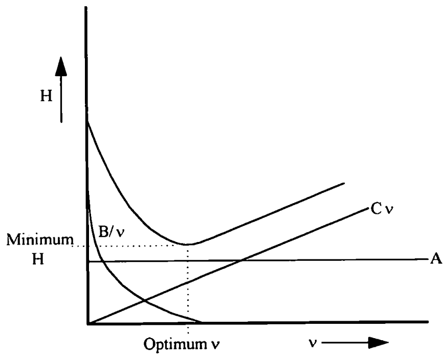
Figure 1.3. The van Deemter plot. The top curve is the total of the three spreading mechanisms.
