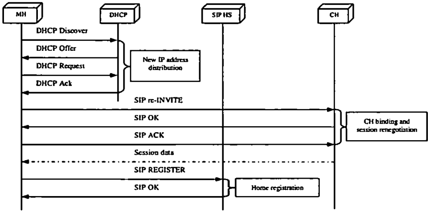
Figure 2.13 SIP mobility: handoff (including location update)
