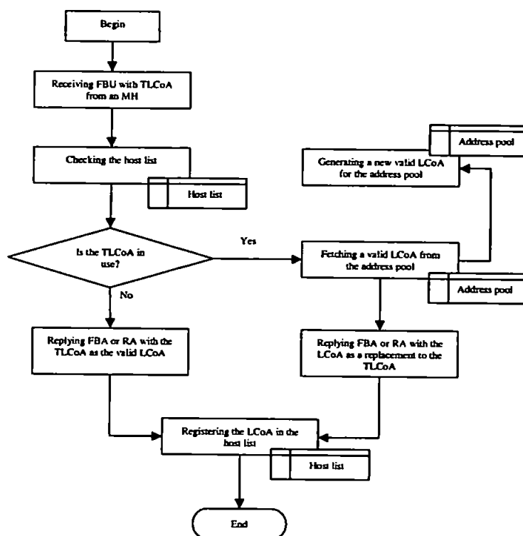
Figure 6.3 PAVER operation at an AR
