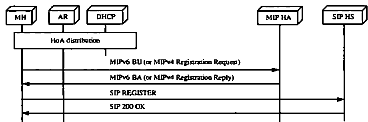
Figure 5.7 LI-MIP-SIP: initial home registration
