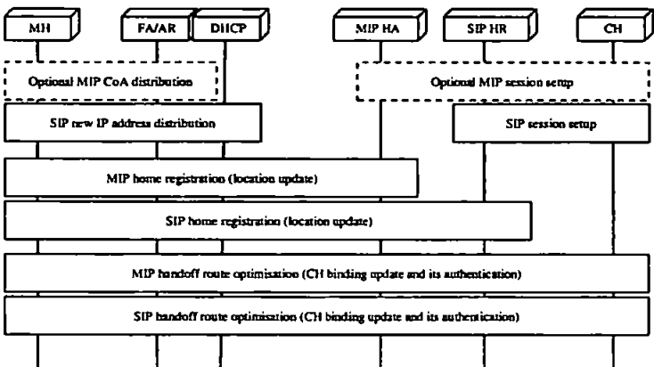
Figure 2.19 Generic mobility signalling block diagram in hybrid MIP-SIP architectures
