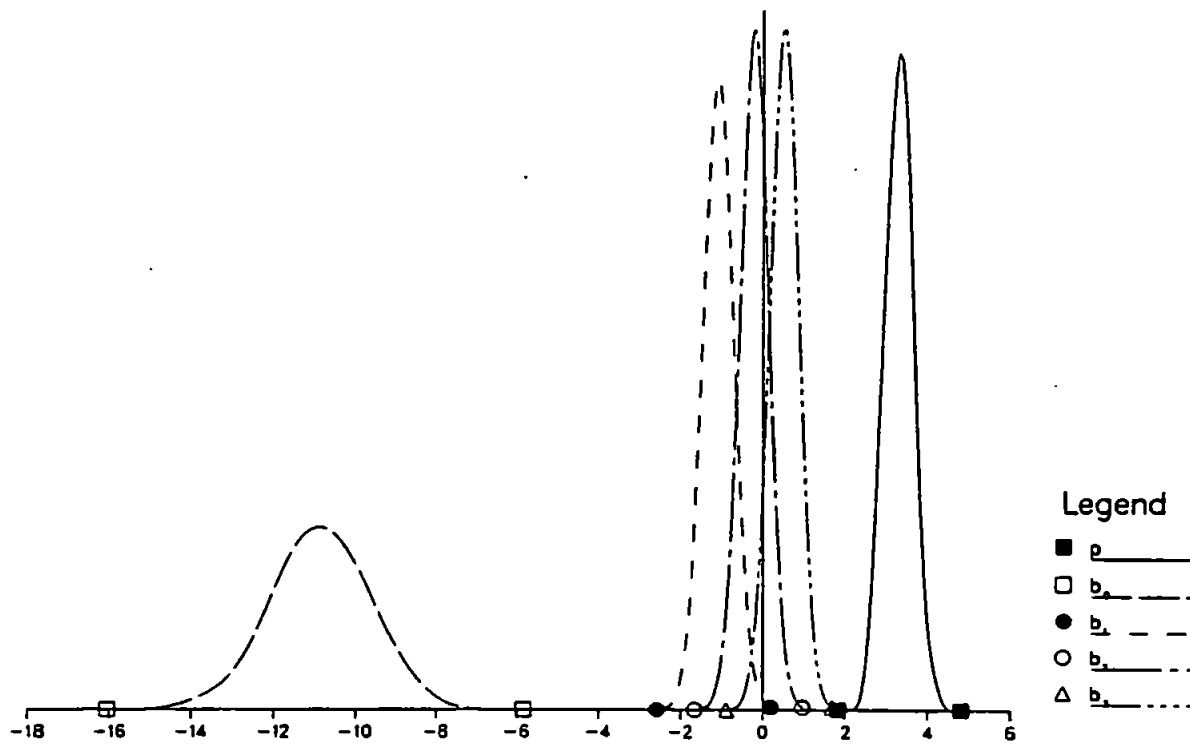
FIGURE 6.8 Marginal densities
