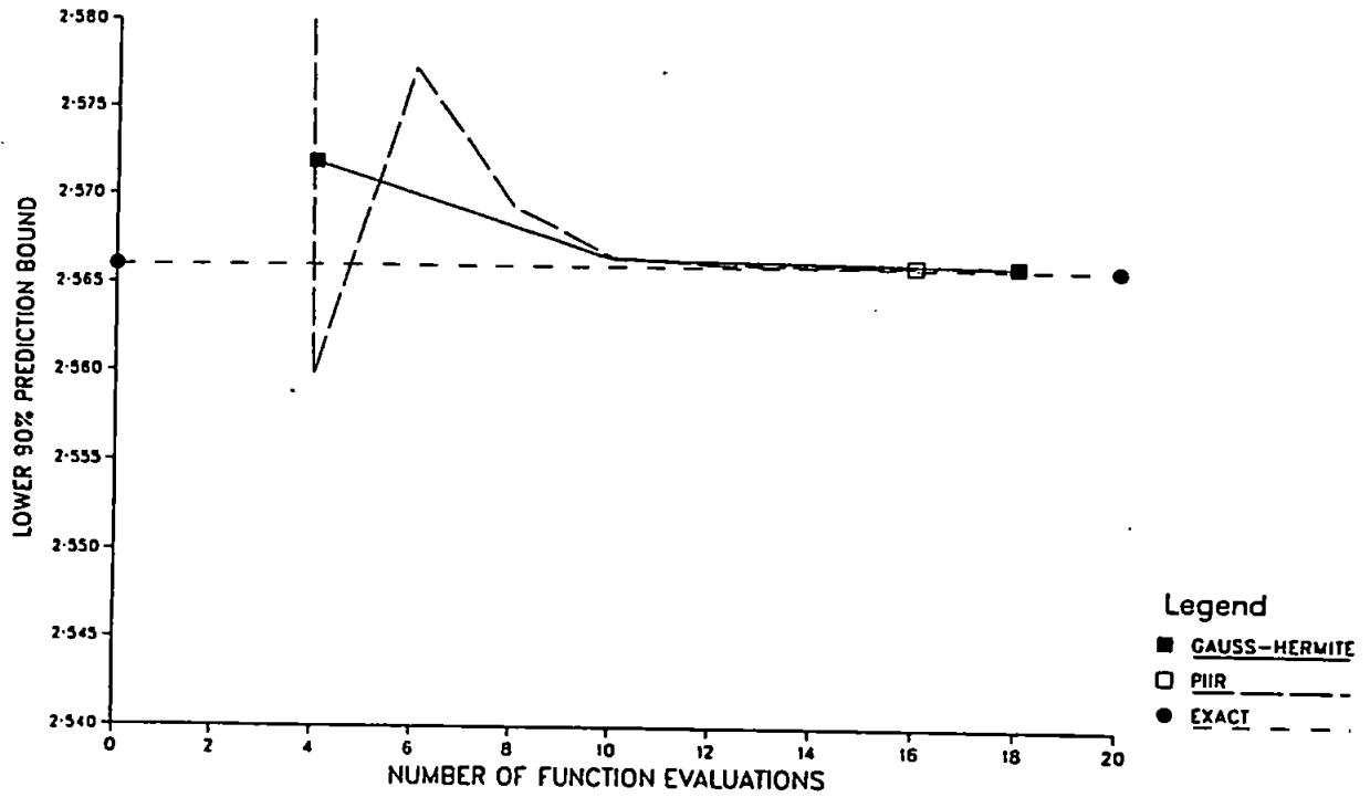
FIGURE 3.10 EXAMPLE 2 WITH PRIOR(2)
