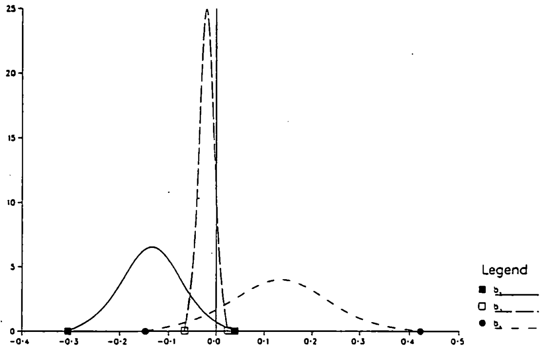
FIGURE 5.21 Marginal densities
