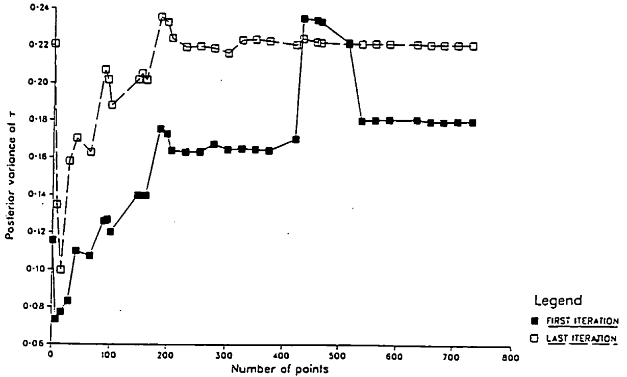
Convergence of posterior variance of \tau
