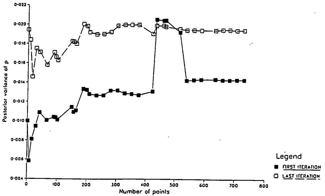
Convergence of posterior variance of p
