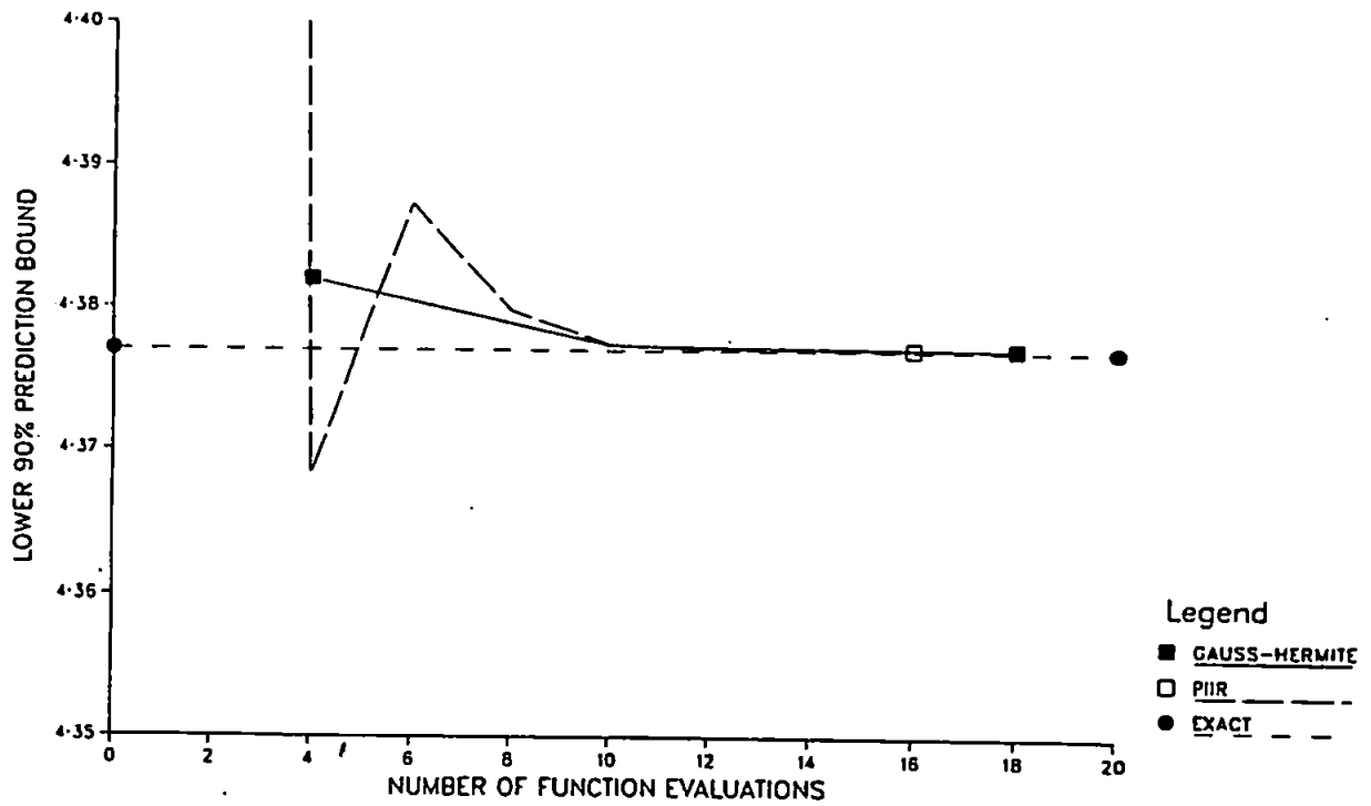
FIGURE 3.10 EXAMPLE 2 WITH PRIOR(2)
