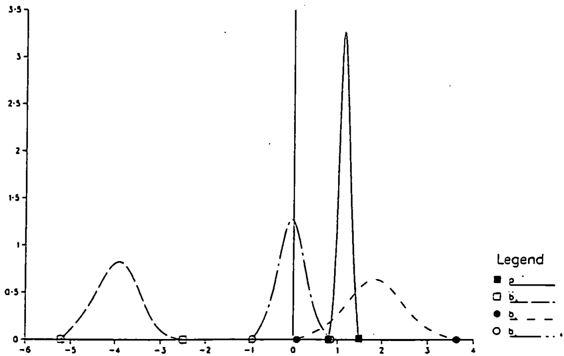
FIGURE 5.22 Marginal densities
