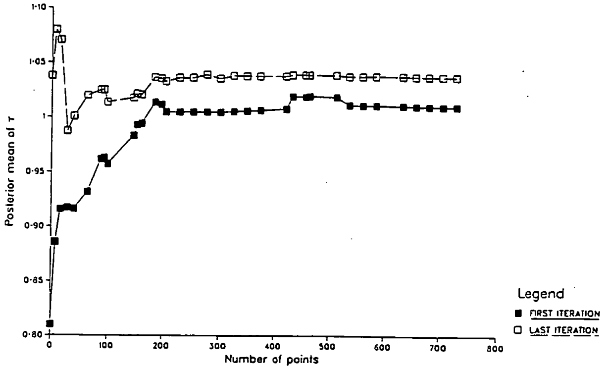
Convergence of posterior mean of \tau
