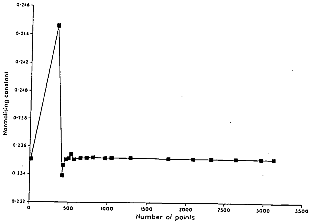
Convergence of normalising constant
