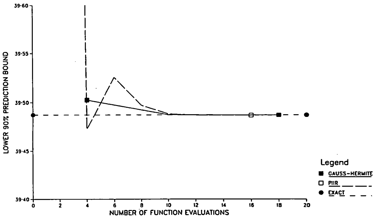
EXAMPLE 1 WITH PRIOR(2)
