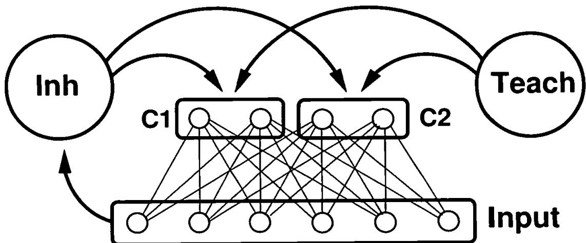
Figure 6.1: A schematic view of the spike-driven network architecture. When considering two classes of stimuli the output units are grouped into two pools each selective to a given class. Additional signals are provided by external inhibitory and teacher populations.
