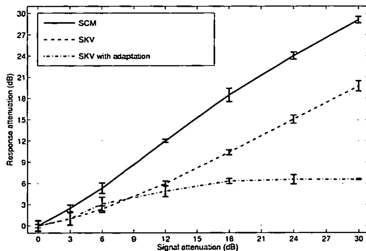
Figure 2.4: Signal attenuation plotted against the attenuation of the RMS activity in the SCM and SKV representations, with and without adaptation. This shows a degree of level independence, see Section 2.4.2
