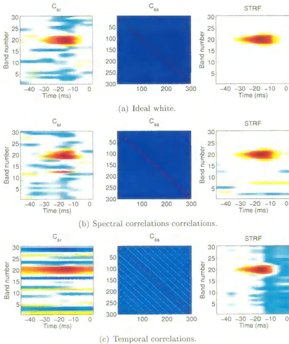
Figure 3.3: Estimate of the example kernel using illustrative stimuli and the methods outlined in Section 3.3.1. Left: the stimulus/response cross-correlation, Centre: the stimulus autocorrelation, Right: the result of correcting the estimate using the correlations in the stimulus. The stimuli are designed to be: Upper: ideal uncorrelated or 'white', Centre: with correlations between frequency bands, Lower: with correlations in time. See Section 3.4.2 for details.
