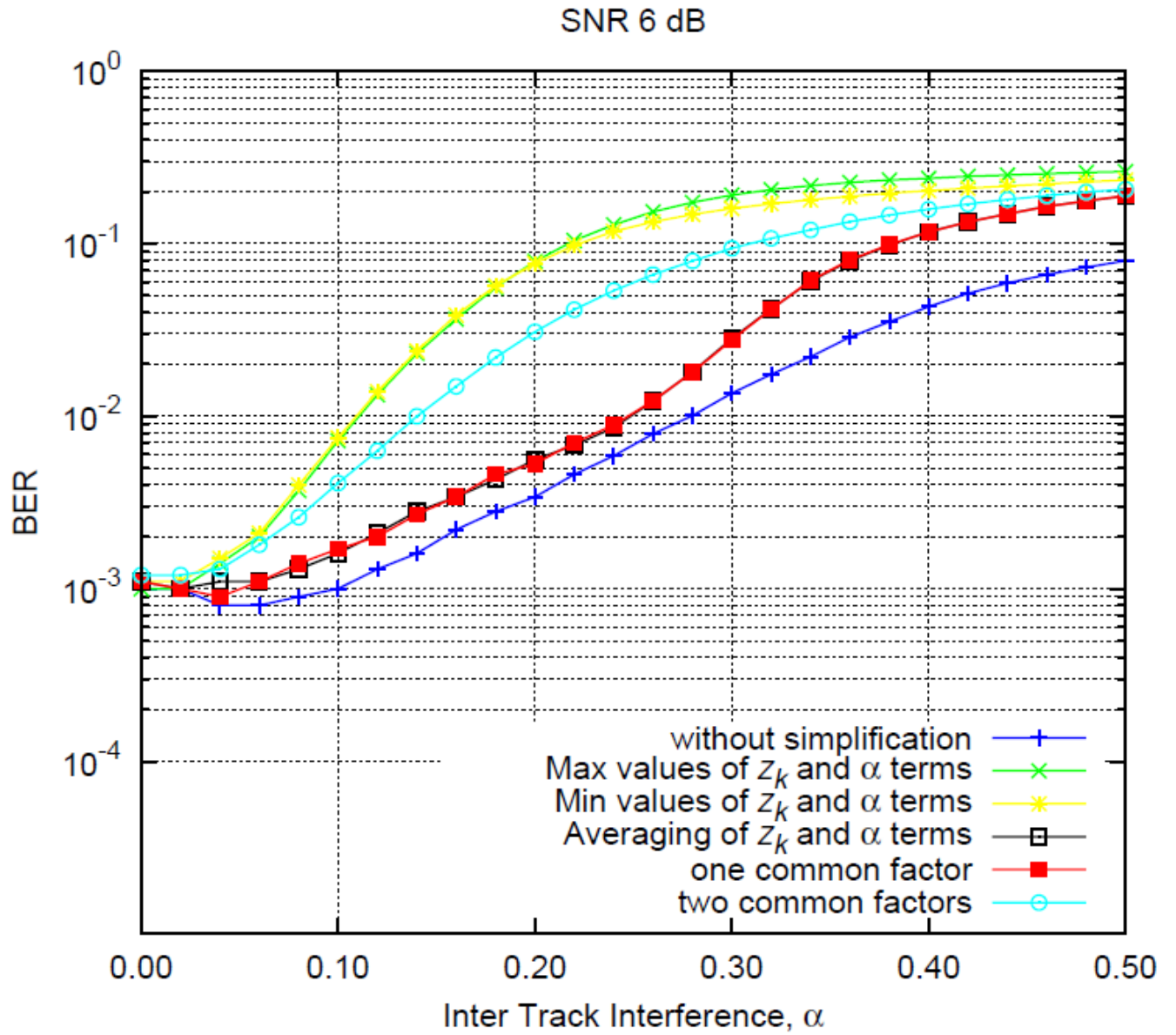
Figure 4.5: BER Performance for Shingled System at 6 dB SNR
