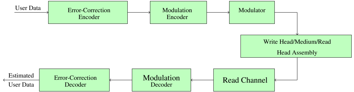
Figure 2.1: Data Storage System Block Diagram [10][11]
