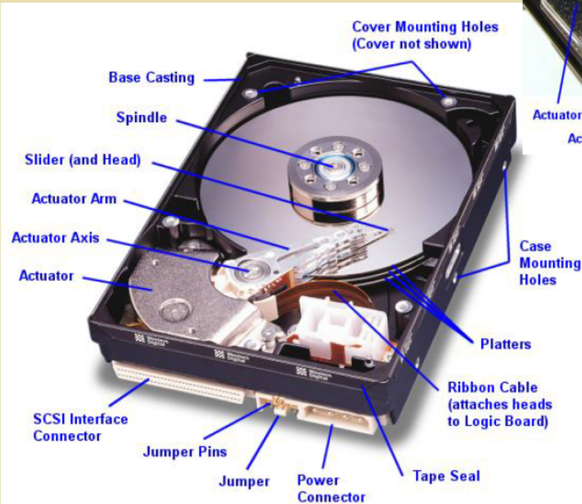
Figure 1.1: Hard Disk Drive Parts [2]
