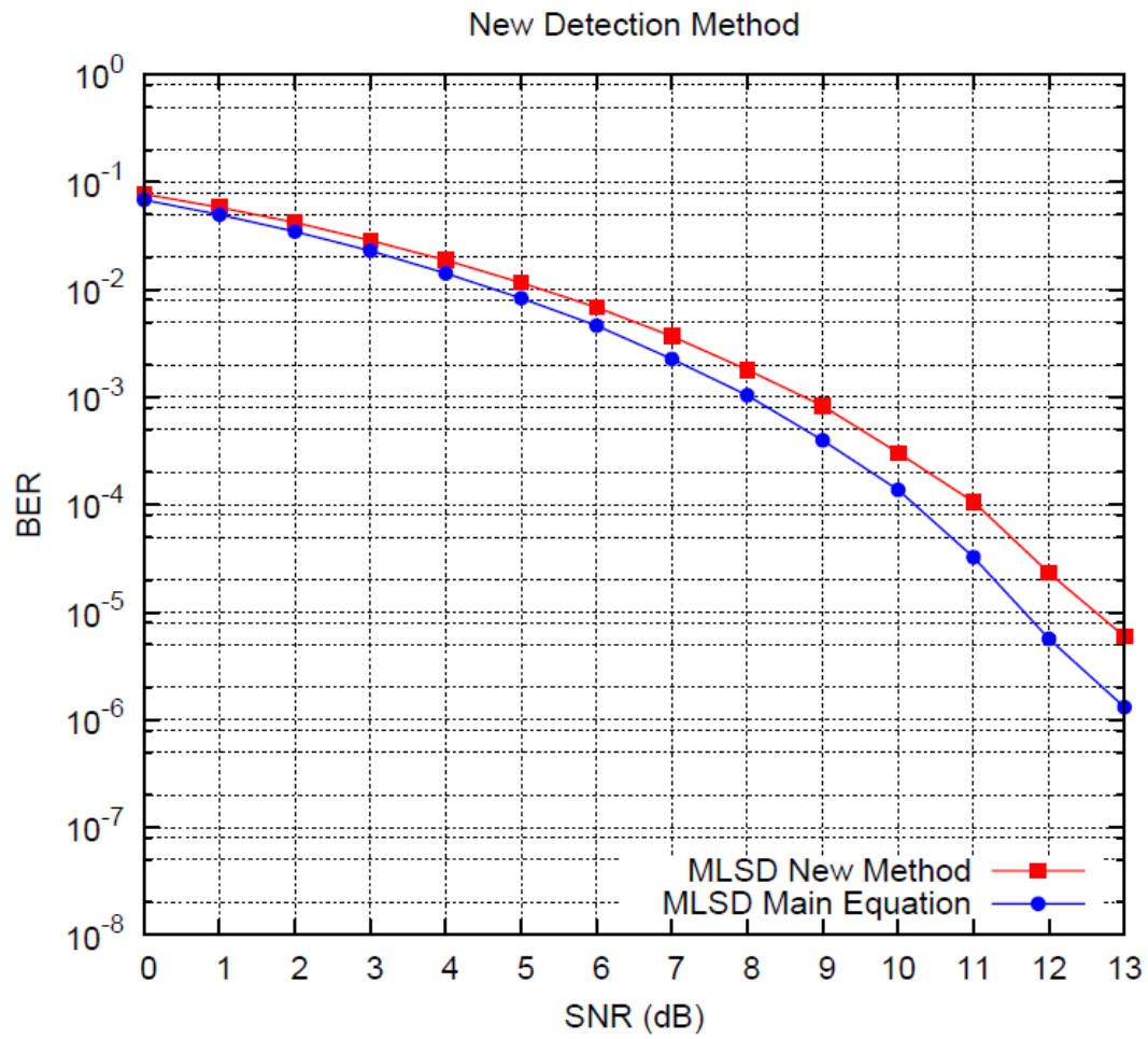
Figure 4.9: BER Performance Comparison
