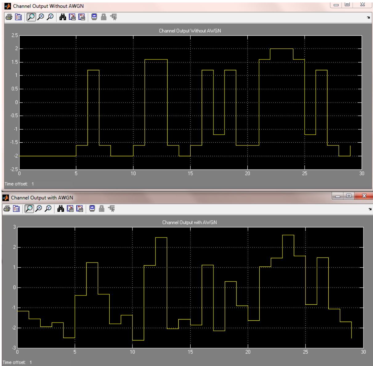
Figure 6.16: PMR Channel Output Without and With AWGN
