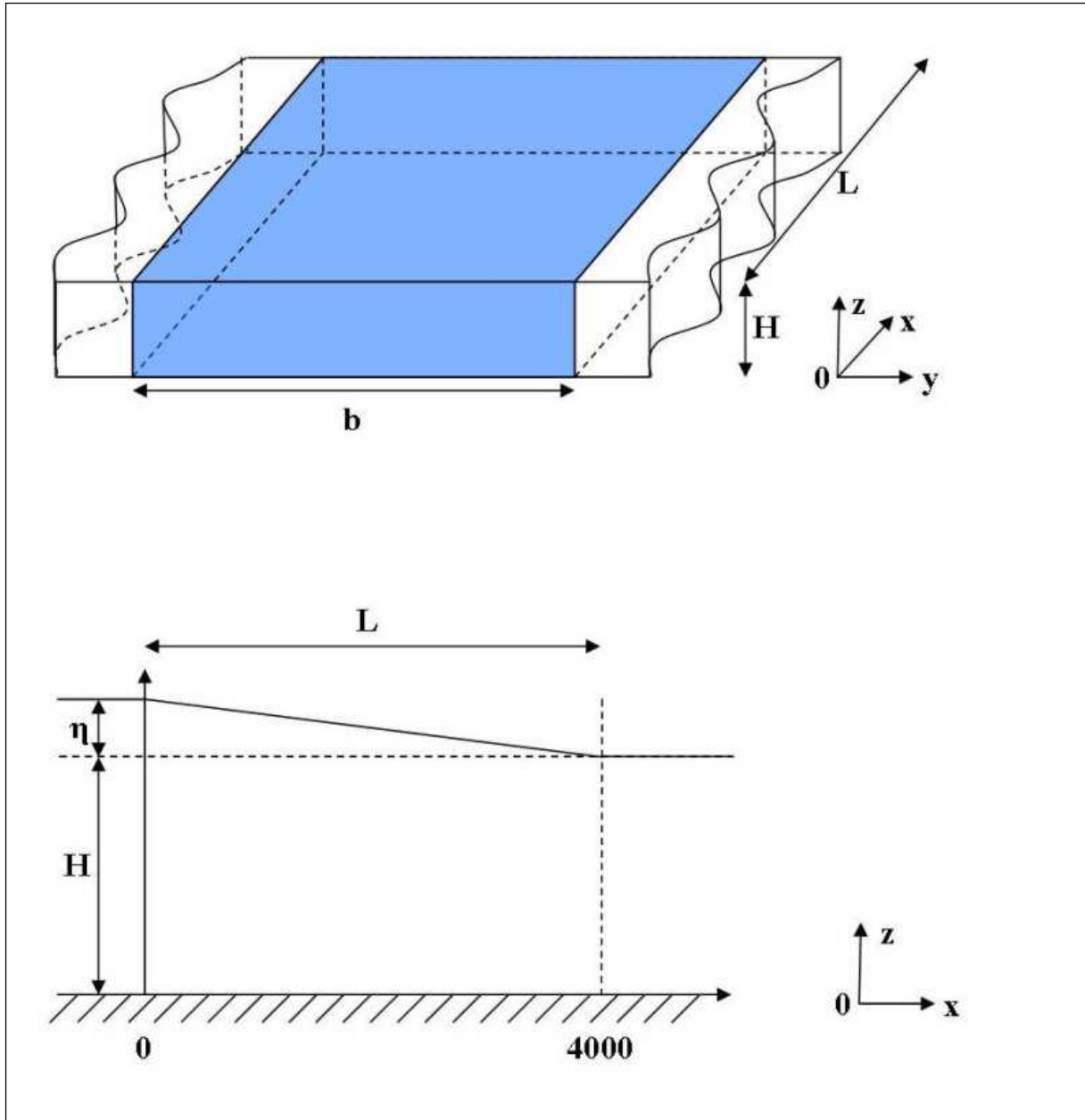
Figure 5: Simplified-channel diagram
