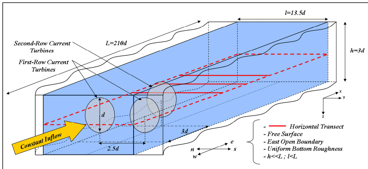
Figure 35: Idealized channel, multi-disc case - This conceptual diagram represents the multi-disc test geometry and dimensions as well as the locations where horizontal transects (red solid lines) have been taken.
