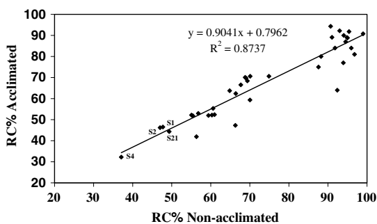
Fig. 3 Correlation between acclimated and non-acclimated frost hardiness expression at -7^{\circ}\text{C} for the selected population
