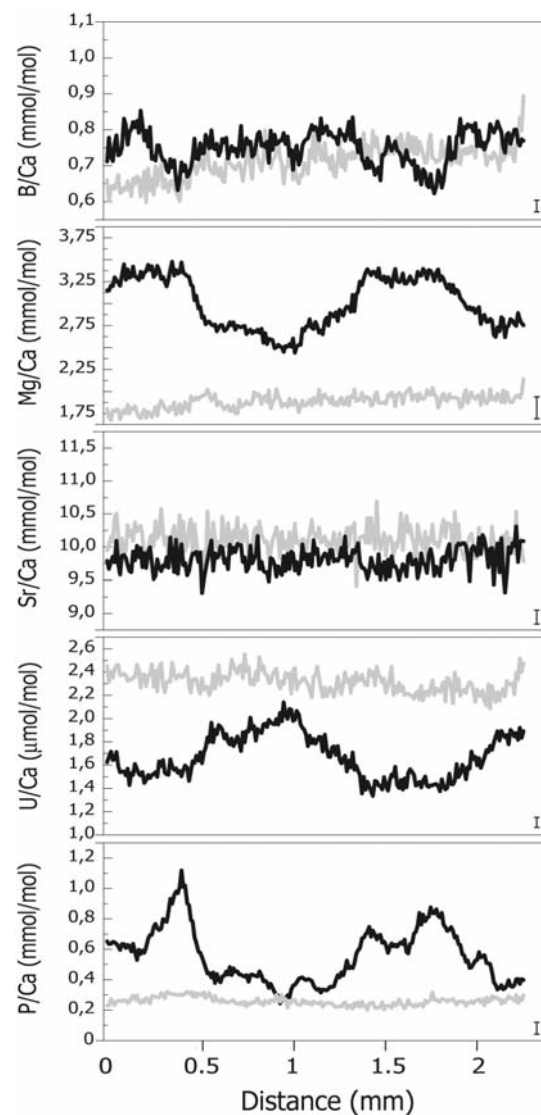
Figure 3. B/Ca, Mg/Ca, Sr/Ca, U/Ca and P/Ca ratios measured along two laser ablation tracks on the transverse sections of the S1 septum. Black and grey lines represent the laser ablation tracks across the centres of calcification (COCs) and the fibrous aragonite (FA), respectively.
