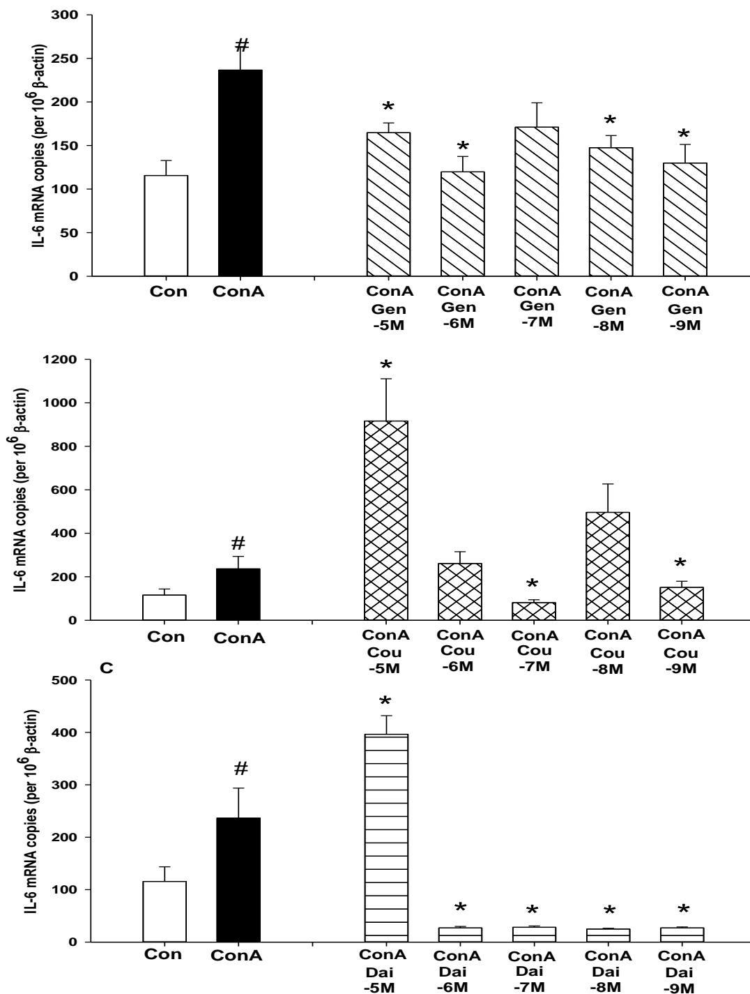
Figure 6.6. Genistein (A), coumestrol (B) and daidzein (C) reduced IL-6 expression in activated Jurkat T cells. Jurkat E6.1 T cells were incubated in combination of conA (10 \mu g/ml), genistein (10 -5 -10 -9 M), coumestrol (10 -5 -10 -9 M) or daidzein (10 -5 -10 -9 M) for 4 days. The expression was assessed by quantitative real time PCR and data normalised to 10 6 copies of \beta -actin and expressed as mean ( \pm SEM). * P<0.05 versus conA treated group, # P<0.05 versus control group.
