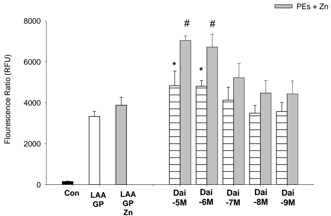
Figure 5.7. Zinc augments the effect of daidzein on osteoblasts mineralisation and differentiation. Saos-2 cells were incubated with daidzein ( 10^{-9} - 10^{-5} M) with or without zinc ( 10^{-5} M) for 18 days. Mineralisation measured using calcein incorporation. Values are expressed as a mean ( \pm SEM) from three experiments. Differences between groups were assessed by one-way analysis of variance. * P < 0.05 versus (LAA+GP) group, # P < 0.05 versus relevant PE treated group.
