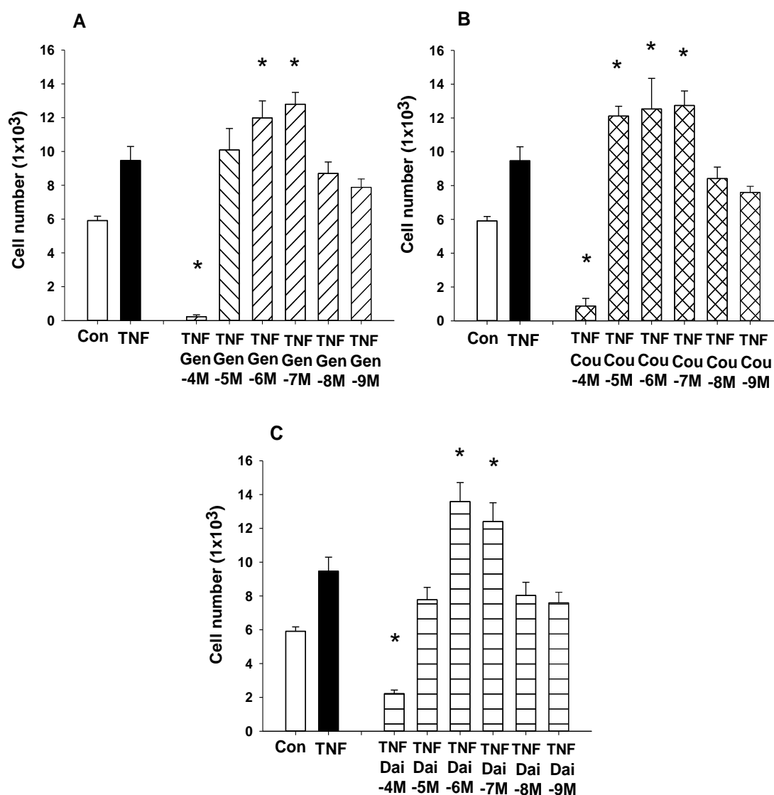
Figure 4.4. Genistein, coumestrol and daidzein ( 10^{-4} M) significantly decreased RAW264.7 cell viability after four days of incubation. All other concentrations had no detrimental effect on monocyte number. RAW264.7 cells treated with TNF- \alpha (50ng/ml) and phytoestrogens ( 10^{-4} - 10^{-9} M), and after four days, the number of viable cells was quantified using an MTS assay. Values are expressed as the mean \pm SEM of 3 separate experiments n=18 , * P < 0.05 versus TNF- \alpha treated group.
