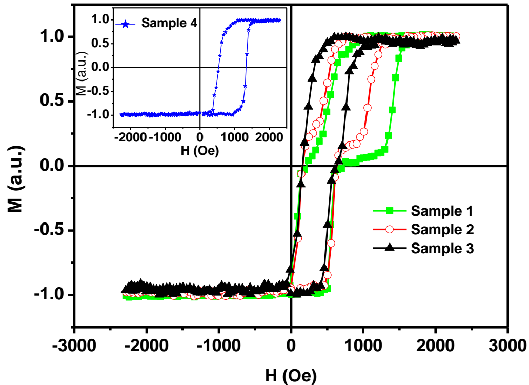
Fig. 5.1. MH loops of four selected samples. Sample 1 has a layer structure \text{SiO}_2/\text{Ta} (5 nm)/CoFe (3.4 nm)/IrMn (5 nm)/CoFeB (3 nm)/Ta (5 nm) annealed at 350 °C for 1 hour. Sample 2 has an identical layer structure as sample 1, but annealed at 250 °C for 1hour. Sample 3 has a layer structure \text{Si}/\text{Ta} (5 nm)/CoFe (3.4 nm)/IrMn (5 nm)/CoFe (3 nm)/Ta (5 nm) annealed at 350 °C for 1 hour. Sample 4 has a layer structure \text{Si}/\text{Ta} (5 nm)/Cu (3.4 nm)/IrMn (5 nm)/CoFeB (3 nm)/Ta (5 nm) with T_A of 350 °C for 1hour. The lower half of the MH loops for samples 1, 2& 3 is the contribution from the CoFe seed layer.
