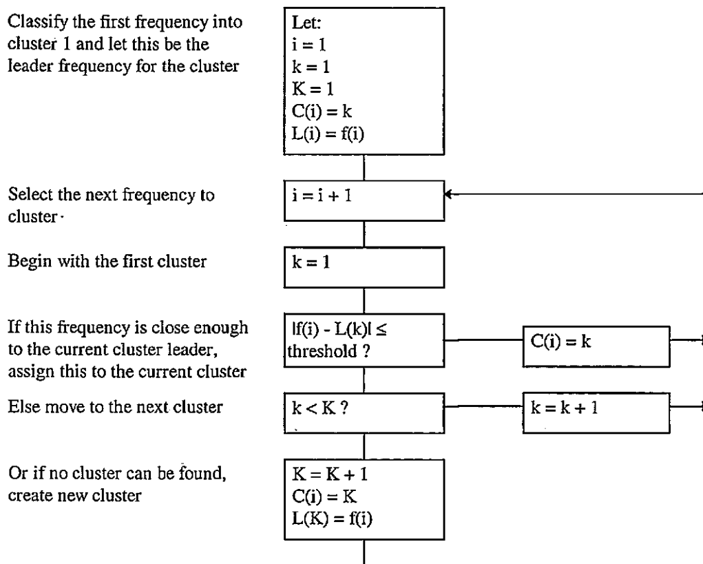
Figure 35. The leader cluster algorithm used to cluster the feature 'frequency'.
