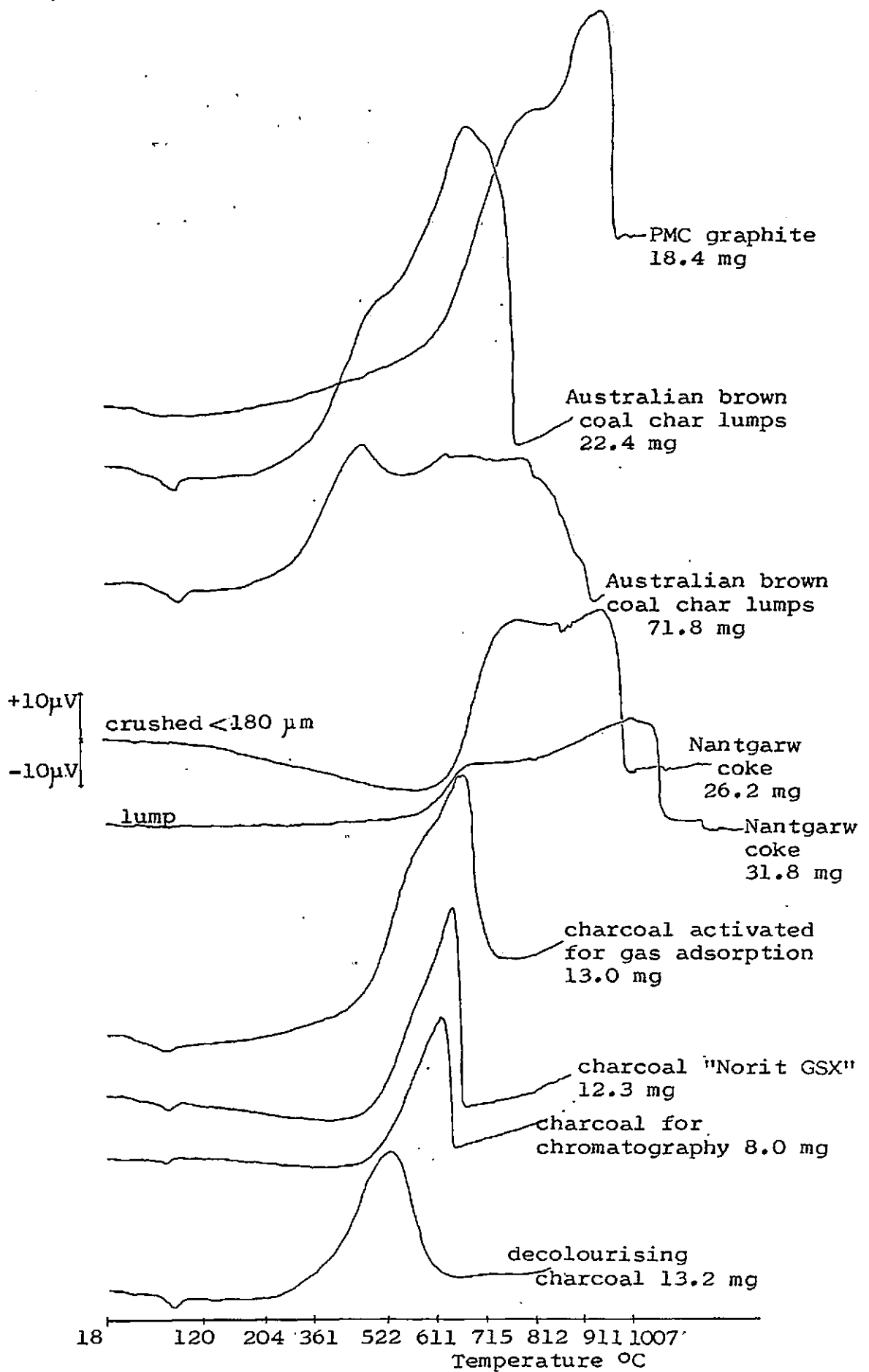
Figure 7.2. DTA of Static Air oxidation of Coke, Char, Charcoals and Graphite under a temperature programme of 5^{\circ}\text{C min}^{-1} .
