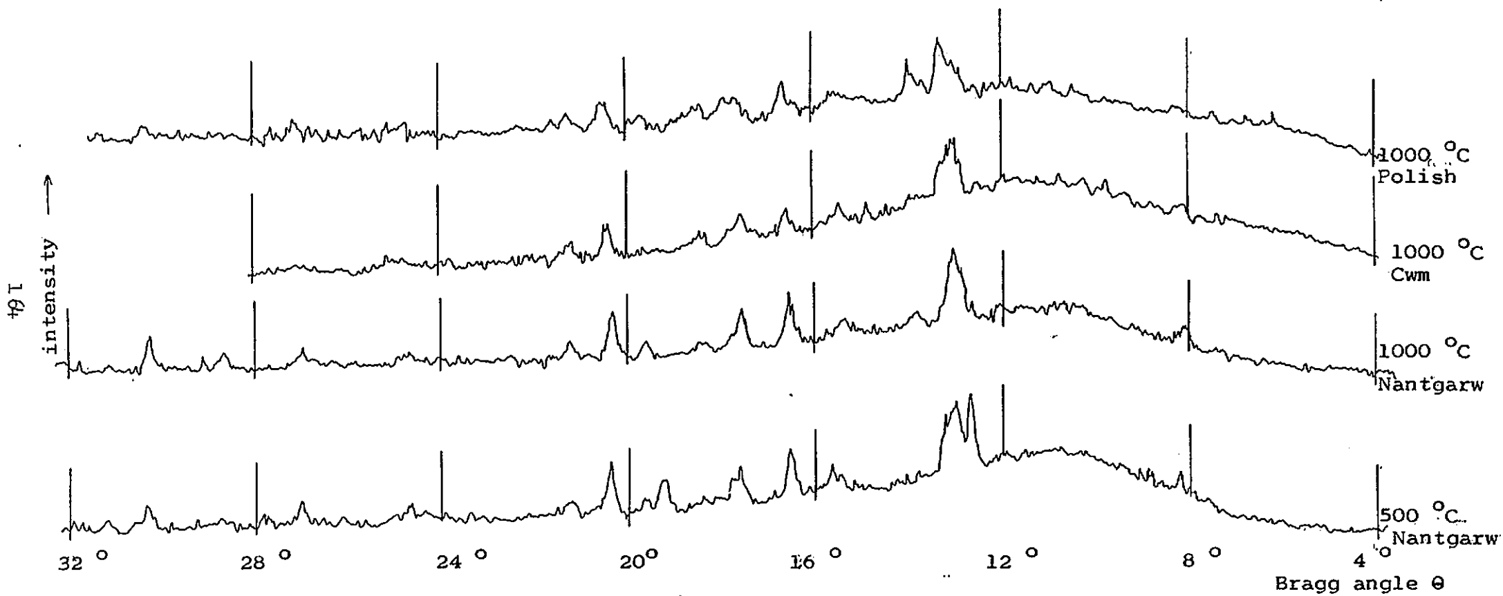
Figure 4.6. X ray powder diffraction traces of coke ash from air burn offs.
