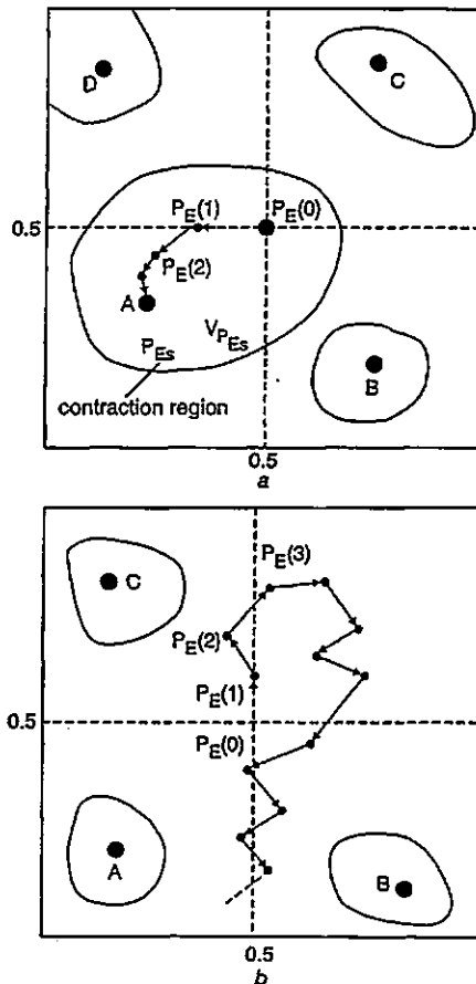
Fig. 2 Visualisation of convergence ( N = 2 )
