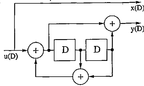
Figure 2.5: RSC(5/7) encoder
