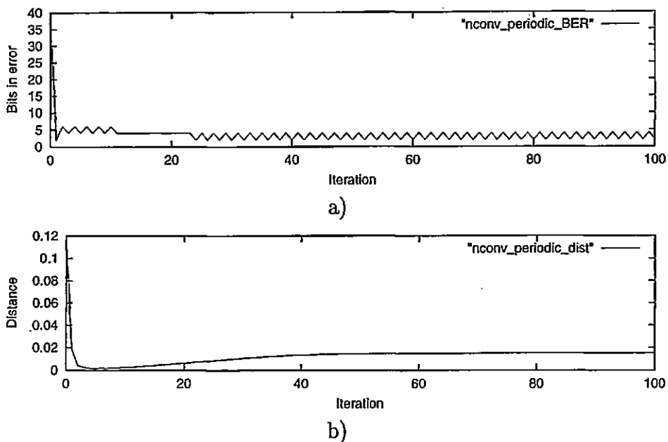
Figure 5.21: Periodic block
