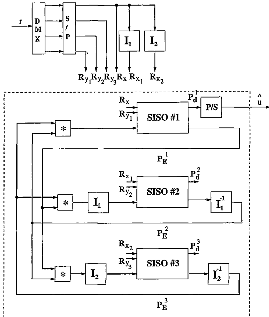
Figure 2.17: 3PCCC decoder
