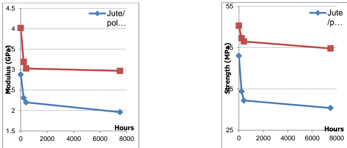
Figure 3: The deterioration of flexural modulus and strength for jute fibre composites exposed to distilled water for 0, 220, 410 or 7500 hours (data from Costa and D’Almeida [53])
