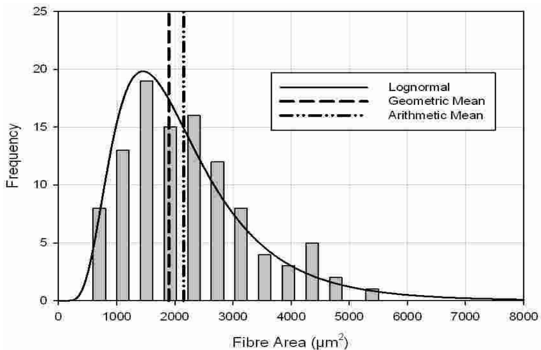
Figure 2: Distribution of fibre cross-sectional areas for jute fibres (Virk data)
