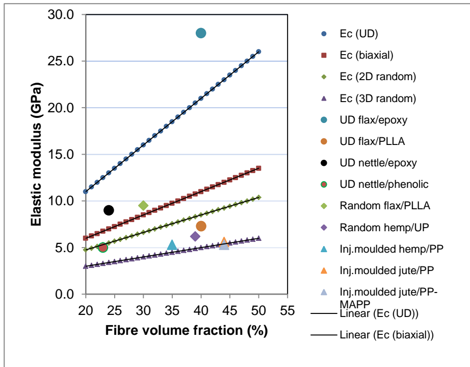
Figure 2: Variation of Young's modulus with fibre orientation plotted against fibre volume fraction (a constant fibre modulus of 50 GPa has been assumed for the trendlines)
