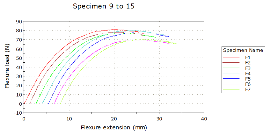
Figure 2. Load vs. deflection curves for glass fibre reinforced composite samples (specimens 1 to 8) and for flax fibre reinforced composite samples (specimens 9-15)
