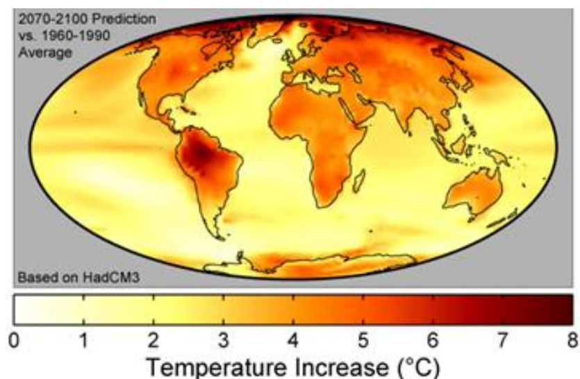
Figure 2.15 Global Warming Predictions for 2070-2100 vs 1960-1990 averages
