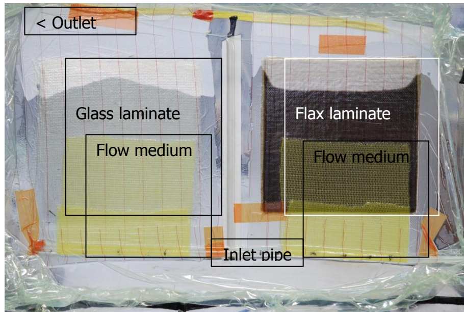
Figure 1. Photograph of experiment set up (each laminate is 200 mm square)
