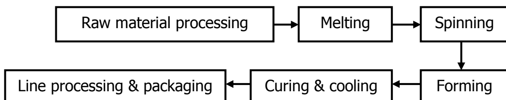
Figure 2. Flow diagram of glass fibre production process.
