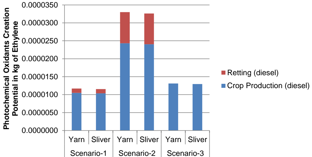
Figure 6.7 Photochemical Oxidants Creation Potential (POCP) for the production of flax sliver and yarn
