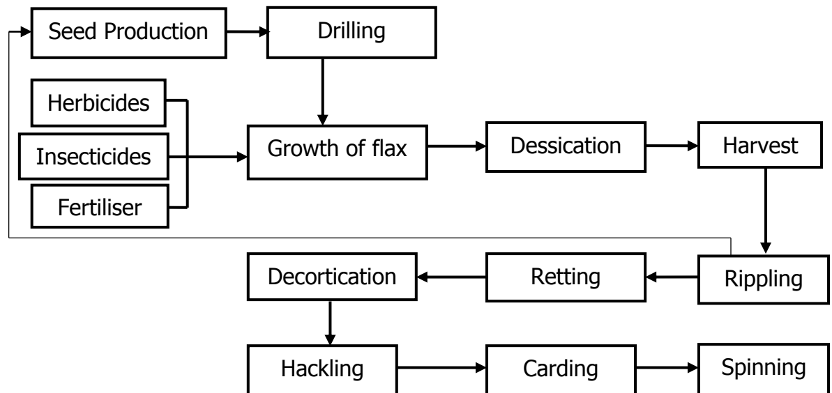
Figure 1. Flow Diagram of Life Cycle of flax fibre as reinforcement for composites.
