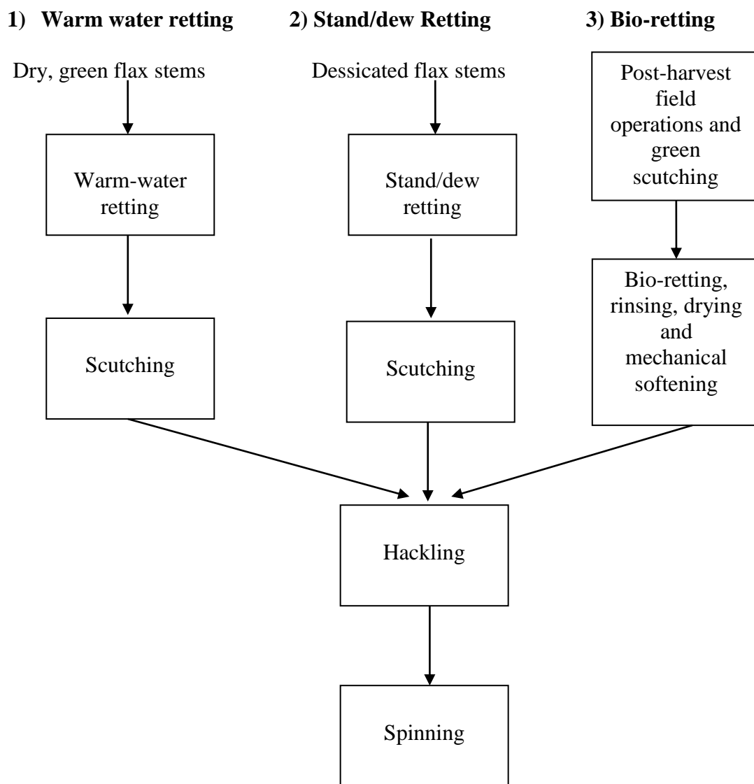
Figure 5.2 Fibre processing stages for different retting methods
