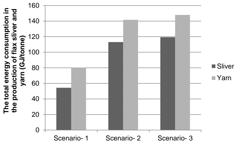
Figure 5.4 The total energy consumption in the production of flax sliver and yarn (GJ/tonne) [86, 87]
