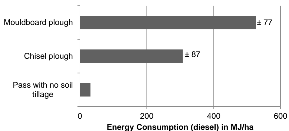
Figure 5.1. Energy consumption in different ploughing methods in MJ/ha
