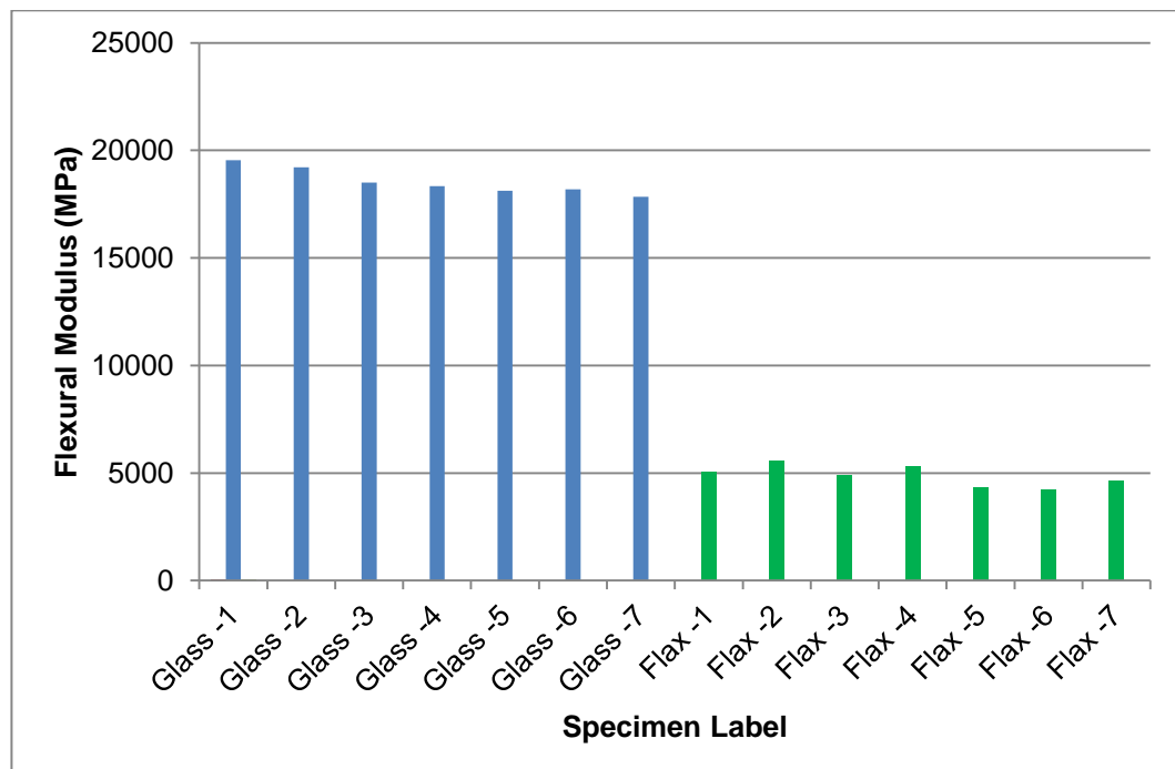
Figure 3. Comparison of flexural moduli for all glass- and flax-reinforced composites
