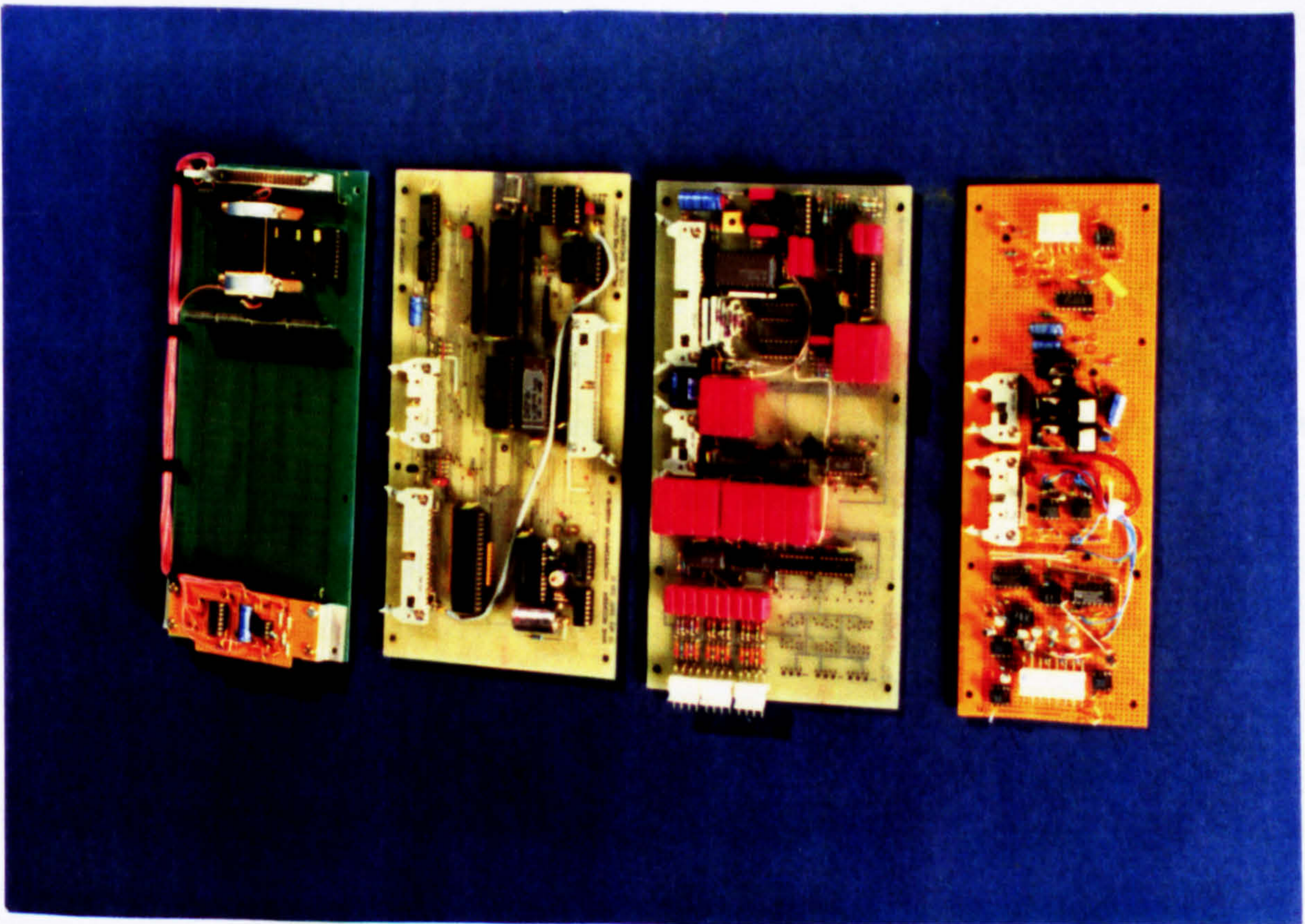
Plate 3 : The four main circuit board assemblies. From the left: data store, microcomputer, signal conditioning, and power supply.
