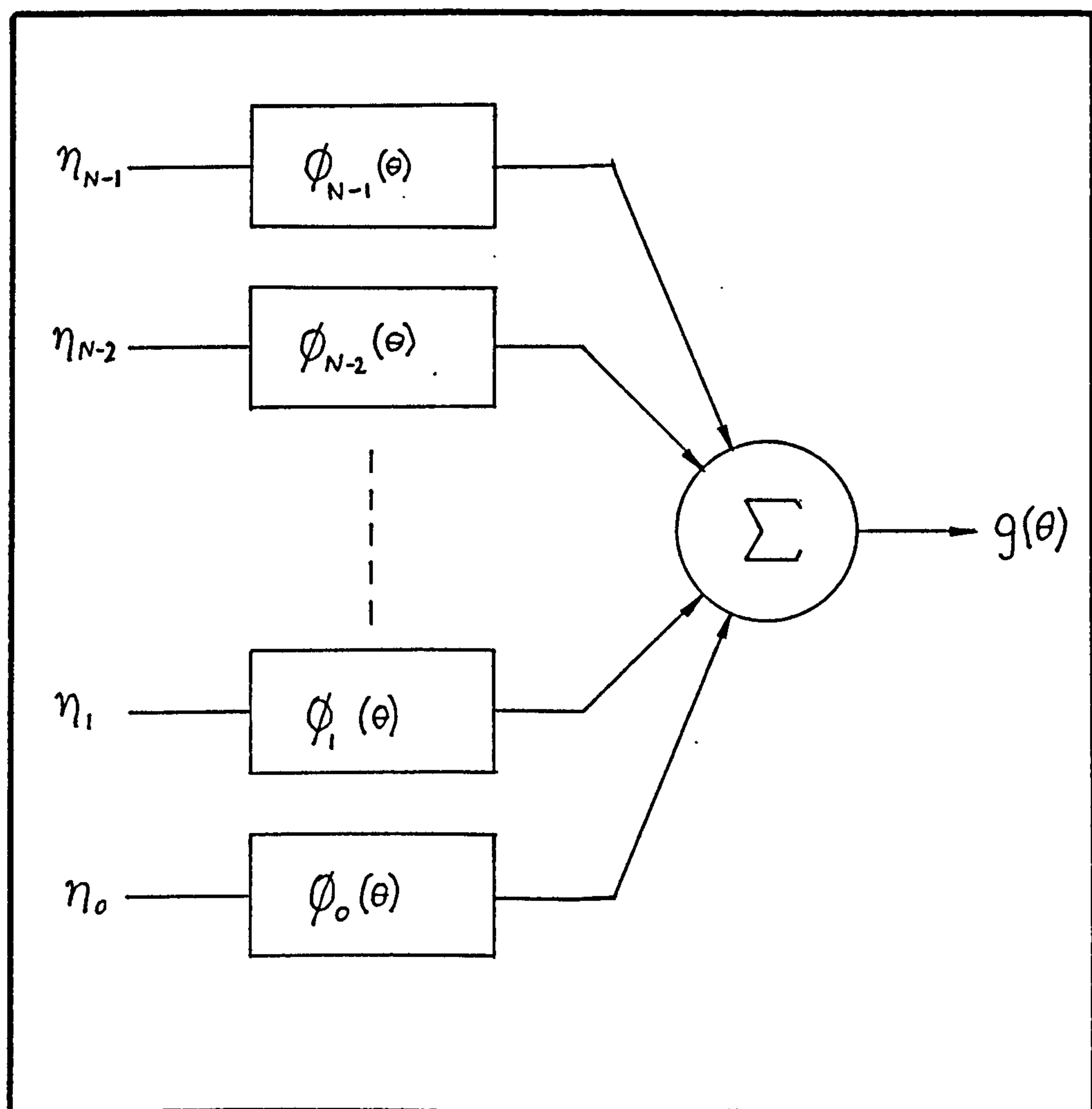
Figure 4.10 : Schematic of the delay-and-sum beamformer
