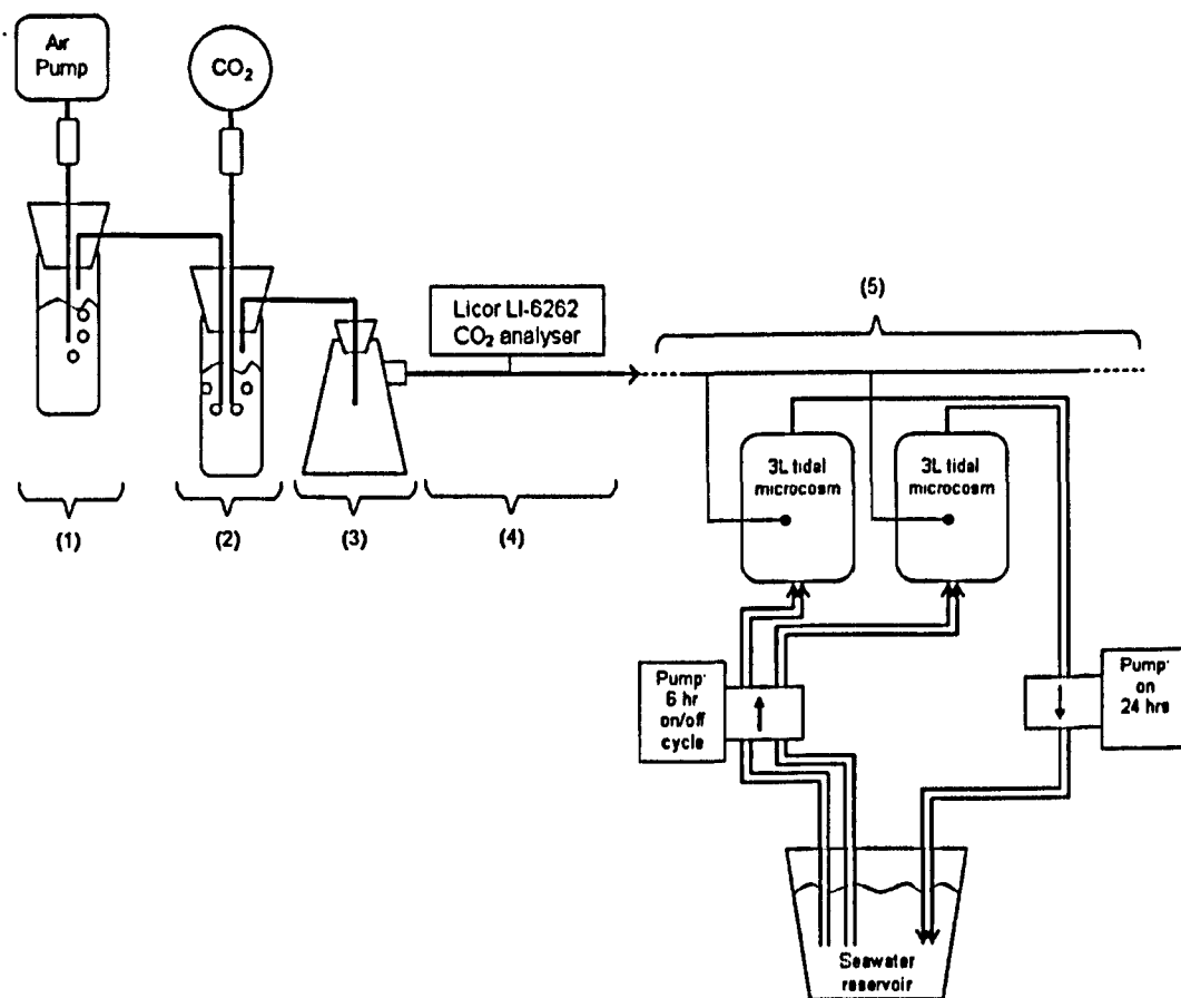
Figure 2.2: Air-CO 2 mixing system consisting of (1) air pumped through a flow meter into a mixing vessel containing soda-lime to remove the CO 2 , (2) pure CO 2 pumped through a flow meter into a mixing vessel along with the CO 2 -free air, (3) mixed high-CO 2 air flows into another vessel to dry the air before (4) passing through a Licor air analyser and on to the microcosms. The tidal system (5) consists of several microcosms connected to the high-CO 2 air or untreated air and seawater, controlled by two pumps: an inflow pump (6 h on/off cycle) and an outflow pump (on 24 h).
