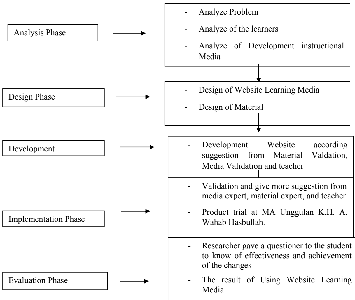
Figure 1. ADDIE Model
