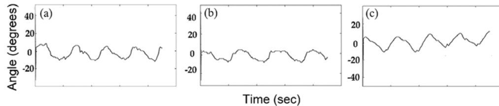
Fig. 2 — Output: (a) Stair descend (b) stair ascend (c) Amputee using a passive hydraulic knee during a straight walk. Notice the change in the hip angles (2a and 2c). This results due to the distinctive limp action of the amputee.
