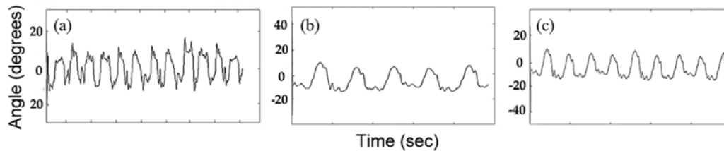
Fig. 1 — (a) Output of earlier SAM system on sound subject with accelerometer (b) Output with 6DOF IMU: straight walk on ground plane (c) straight fast walking on ground plane
