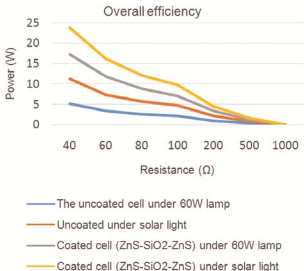
Fig. 2 — FLIR Comparison graph of coated and uncoated solar panel
