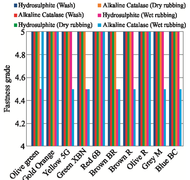
Fig. 5 — Comparison of wash and dry/wet rub fastness
