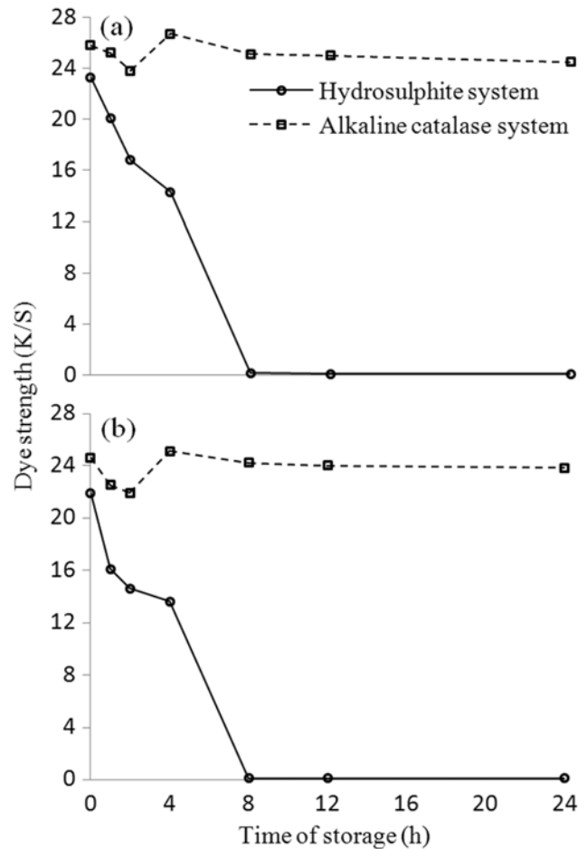
Fig. 3 — Stability of dye baths in (a) absence and (b) presence of dye
