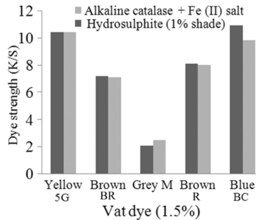
Fig. 2 — Comparison of dye strength on cotton in hydrosulphite system for 1% shade and in alkaline catalase based reduction baths for 1.5% shade
