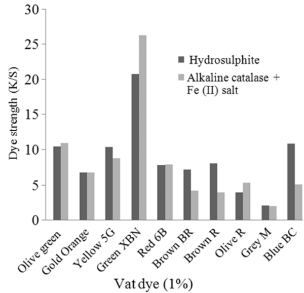
Fig. 1 — Comparison of dye strength on cotton in hydrosulphite and alkaline catalase based reduction baths for 1% shade
