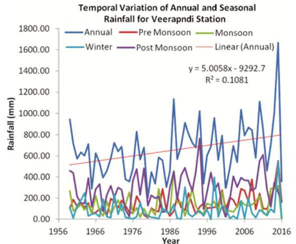
Fig. 9 — Temporal variation of annual and seasonal rainfall for Veerapandi station
