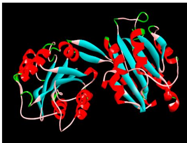
Fig. 2 — 3D structure of the protein 4CN8
