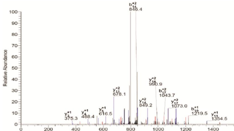
Fig. 1 — Peptide sequence of NPM1 from the results of LC/MS/MS. The peptide sequence “ADKDYHFKVDNDENEHQLSLR” was shown to identify NPM1 by using two-dimensional LC/MS/MS
