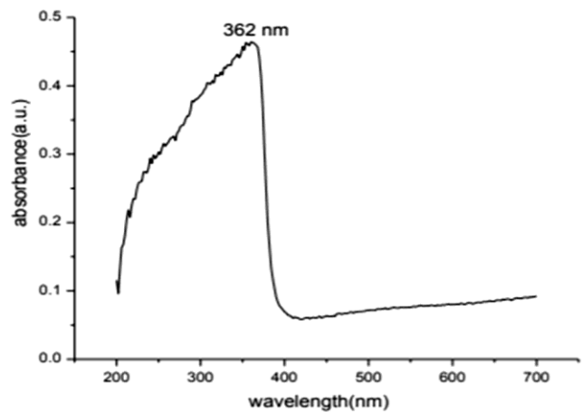
Fig. 1 — UV-visible of synthesized ZnO nanoparticles
