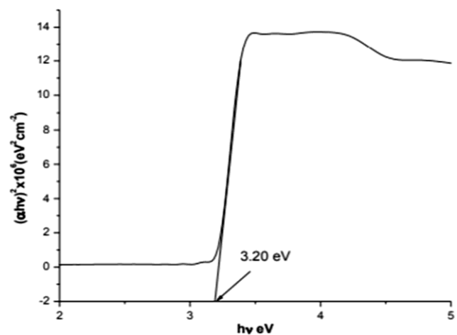
Fig. 2 — Tauc plot for determination of band gap
