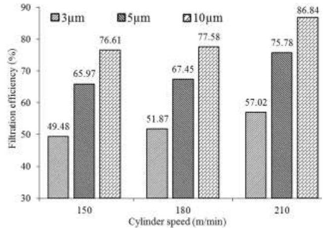
Fig. 3 — Relation between cylinder speed and filtration efficiency
