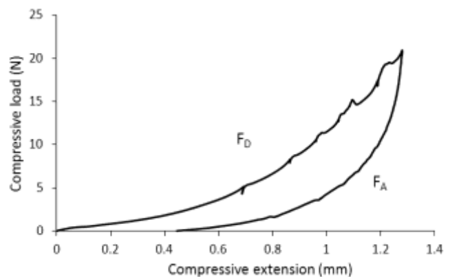
Fig.1 — Typical load elongation curve
