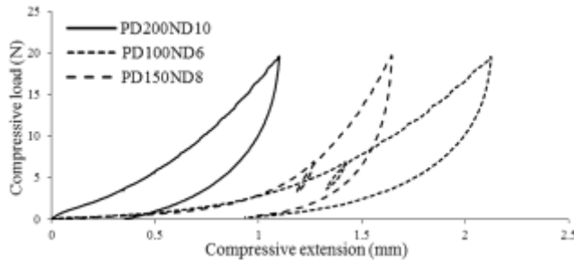
Fig. 4 — Compression and compressional resilience at different cylinder speed
