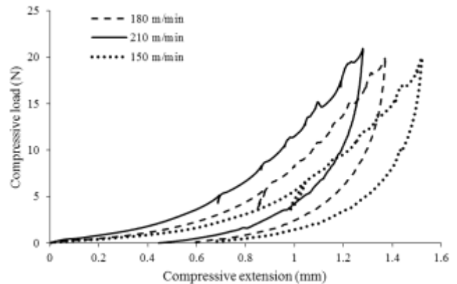
Fig. 2 — Compression and recovery behavior at different cylinder speed
