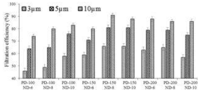
Fig. 5 — Filtration efficiency of 3, 5 and 10 µm particle with different punching parameters
